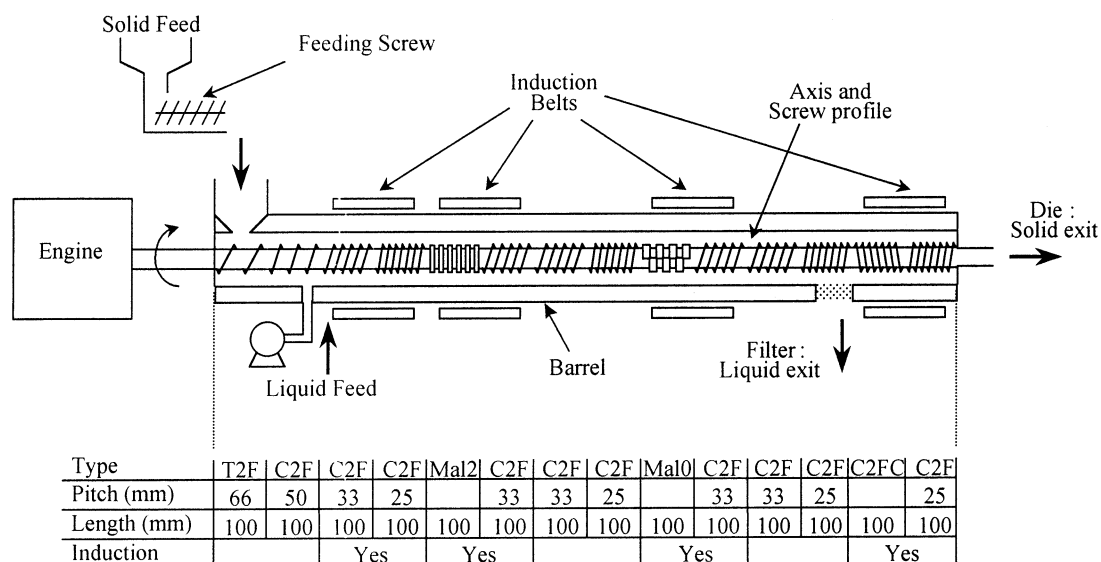
Fig. 1. Global process in a modified CLETRAL BC45 TSE.
