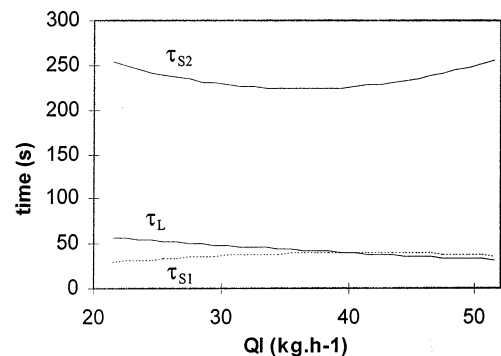
Fig. 8. Influence of Q_L on mean residence times at central functioning point.
