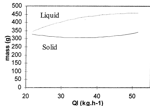
Fig. 9. Influence of Q_L on internal mass at central functioning point.
