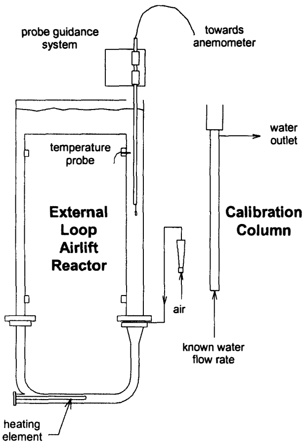
Figure 2 — Experimental set-up.
