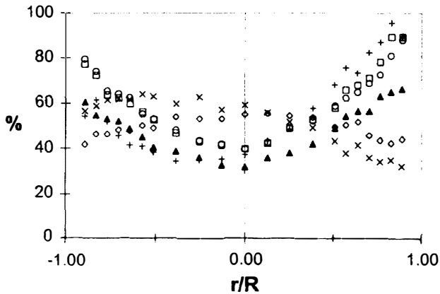
Figure 9 — Turbulence intensity (+ z/D = 2.6 , \blacktriangle z/D = 5.3 , \square z/D = 7.9 , \circ z/D = 10.6 ) and bubble association ratio ( \times z/D = 2.6 , \diamond z/D = 7.9 ) at superficial gas velocity U_G = 0.068 m/s.
