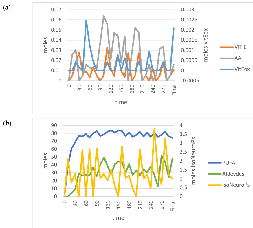
Figure 6. Time-dependent trends (300 min) of the main OUTPUTs obtained by applying the VENSIM software to the standard model when input PUFA increased ( >55.5 moles). (a) AA, Vit E and Vit Eox; (b) PUFA, Aldehydes and IsoNeuroPs. Abbreviations: AA, ascorbic acid; IsoNeuroPs, Iso- and neuroprostanes; PUFA, polyunsaturated fatty acids; Vit E, vitamin E; Vit Eox, oxidised vitamin E.
