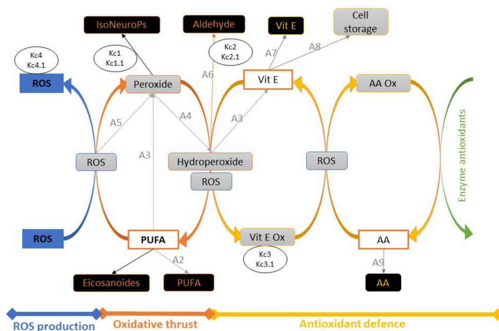
Figure 3. Schematic representation of the model, with INPUTs and OUTPUTs in white and black boxes, respectively. Intermediate OUTPUTs are shown in grey boxes and result from molecular components (substrates and products) and sub-model interactions. The symbols A1–A9 represent the metabolic pathways generating intermediate outcomes (see Section 2.1.3), and Kc1–4 and Kc1.1–4.1 are compensatory rates introduced after model verification by in vivo experimental data (see Section 2.2). Abbreviations: AA, ascorbic acid; AA ox, oxidised ascorbic acid; PUFA, polyunsaturated fatty acids; ROS, reactive oxygen species; Vit E, vitamin E; Vit E ox, oxidised vitamin E.
