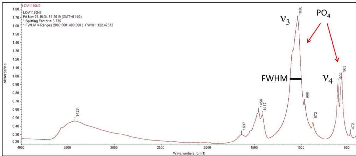
Fig. 2. FTIR spectrum of a natural enamel aliquot from Lovedale (LOV1180).
