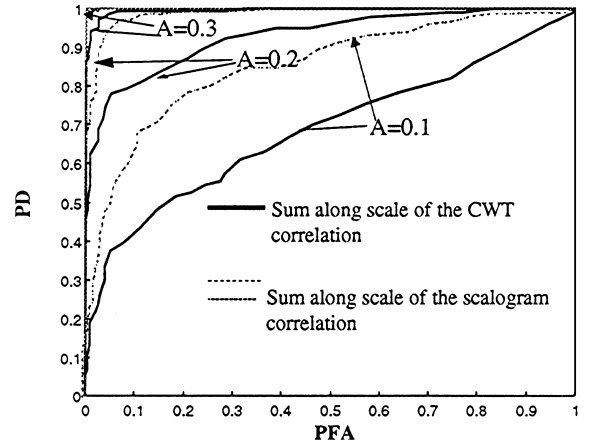
Fig. 13. ROC curves for detectors \Gamma_2(\tau) and \Gamma_4(\tau) (white multiplicative noise).
