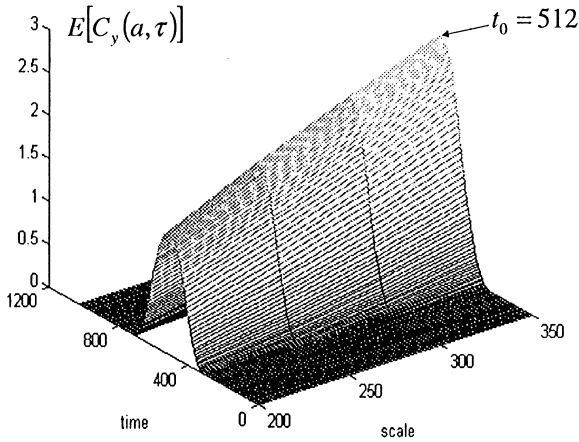
Fig. 7. Ramp signature ( A = 0.4, t_0 = 512, a_0 = 200 ) with symmetrical Haar wavelet.
