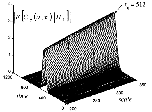
Fig. 3. Step signature ( A = 0.4, t_0 = 512 ) with FDG wavelet.
