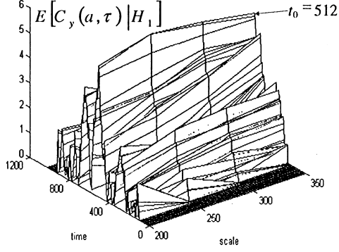
Fig. 4. CWT of a step ( A = 0.4, t_0 = 512 ) embedded in multiplicative noise with Haar wavelet.
