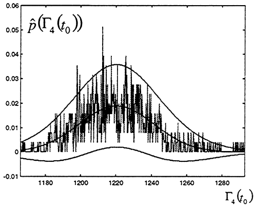
Fig. 19. Histogram of \Gamma_4(t_0) and fitted Gaussian pdf with 95% confidence intervals.
