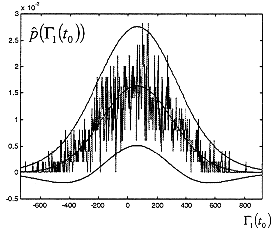
Fig. 16. Histogram of \Gamma_1(t_0) and fitted Gaussian pdf with 95% confidence intervals.
