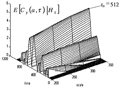
Fig. 5. CWT of a step ( A = 0.4, t_0 = 512 ) embedded in multiplicative noise with FDG wavelet.
