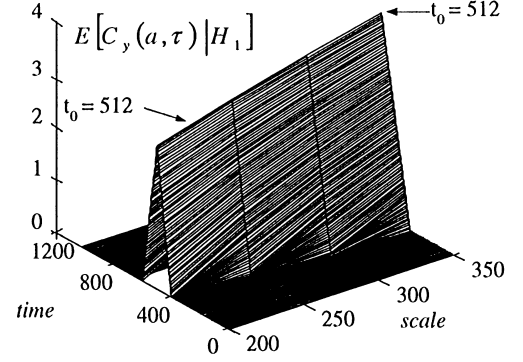
Fig. 2. Step signature ( A = 0.4, t_0 = 512 ) with symmetrical Haar wavelet.
