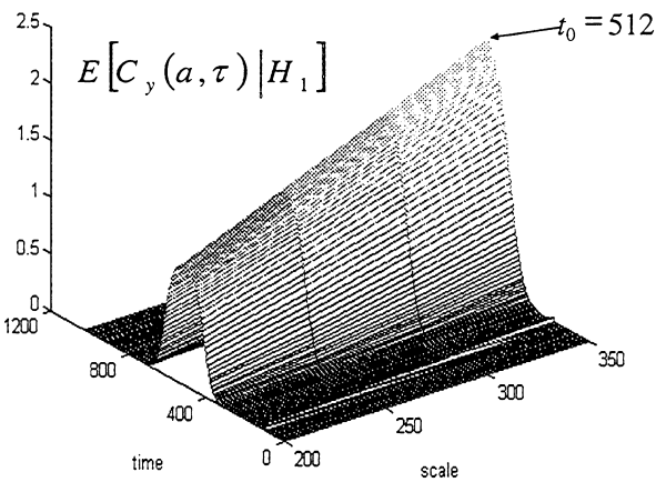
Fig. 8. Ramp signature ( A = 0.4, t_0 = 512, a_0 = 200 ) with FDG wavelet.
