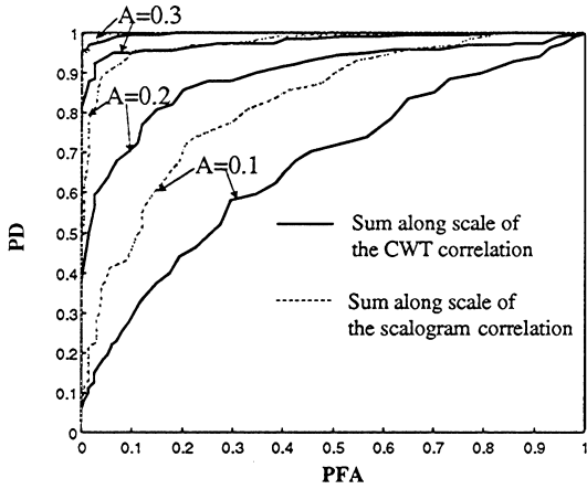
Fig. 15. ROC curves for detectors \Gamma_2(\tau) and \Gamma_4(\tau) (colored multiplicative noise).
