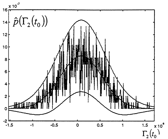
Fig. 17. Histogram of \Gamma_2(t_0) and fitted Gaussian pdf with 95% confidence intervals.
