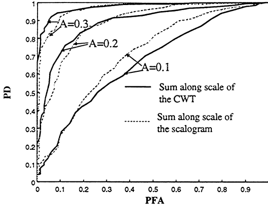
Fig. 14. ROC curves for detectors \Gamma_1(\tau) and \Gamma_3(\tau) (colored multiplicative noise).
