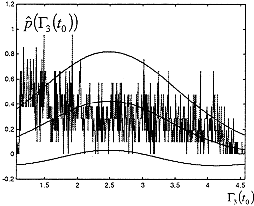
Fig. 18. Histogram of \Gamma_3(t_0) and fitted Gaussian pdf with 95% confidence intervals.
