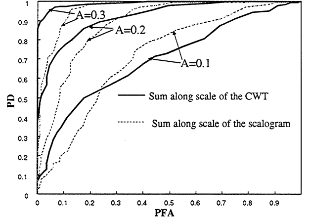
Fig. 12. ROC curves for detectors \Gamma_1(\tau) and \Gamma_3(\tau) (white multiplicative noise).
