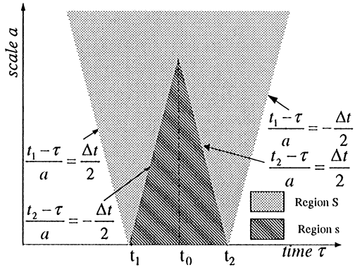
Fig. 6. Support of smoothed change signature ( a_0 \neq 0 ).
