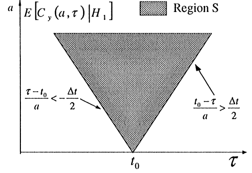
Fig. 1. Support of AC signature ( a_0 = 0 ).
