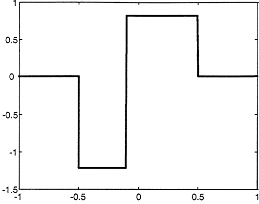
Fig. 11. Optimal wavelet for an AC embedded in white multiplicative noise ( A = 0.5 ).
