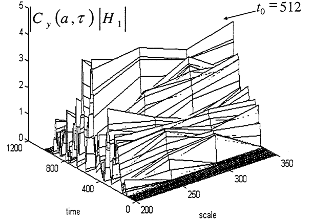
Fig. 9. CWT of a ramp ( A = 0.4, t_0 = 512, a_0 = 200 ) embedded in multiplicative noise with Haar wavelet.
