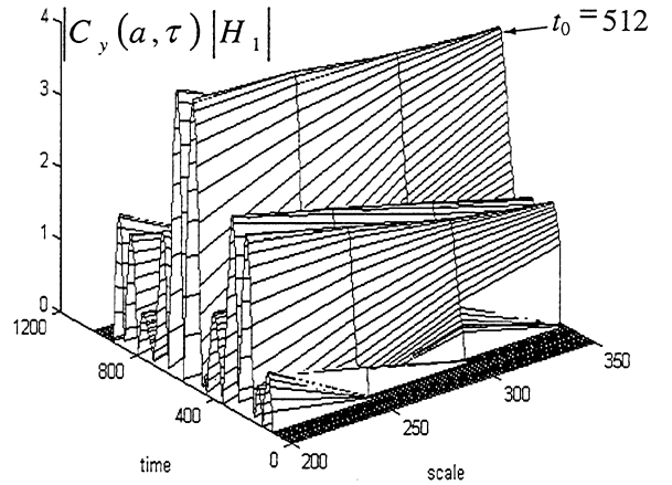
Fig. 10. CWT of a ramp ( A = 0.4, t_0 = 512, a_0 = 200 ) embedded in multiplicative noise with FDG wavelet.
