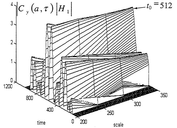
Fig. 10. CWT of a ramp ( A = 0.4, t_0 = 512, a_0 = 200 ) embedded in multiplicative noise with FDG wavelet.
