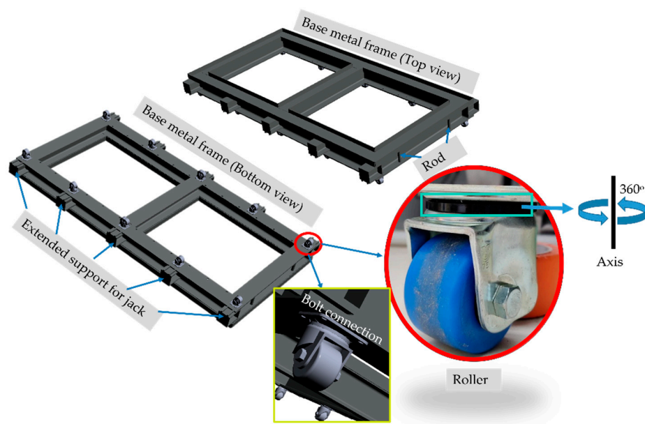
Figure 2. Metallic frame used at the base of the building model.
