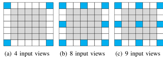
Fig. 7. Three types of input view configurations for NeRF [21], blue squares are input views for training and gray squares are views to be inferred.
