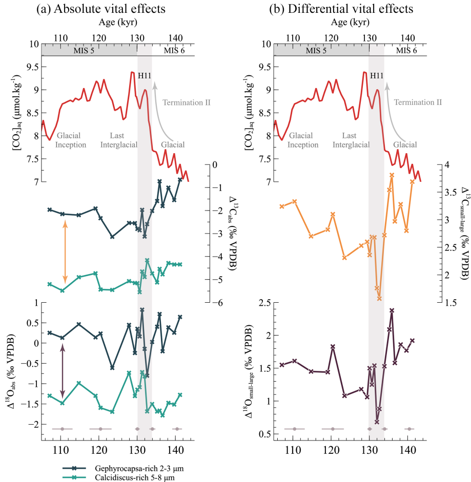
Figure 3. Expression of the coccolith vital effects, both absolute (a) and differential (b), across Termination II. Panel (a): the magnitude of the coccolith absolute vital effect seems to be dependent on coccolith size. Arrows in panel (a) represent the differential vital effects represented in the associated panel (b): the differential vital effect in both carbon and oxygen isotopes is less marked during the interglacial with high aqueous CO 2 concentrations than during the glacial maximum.
