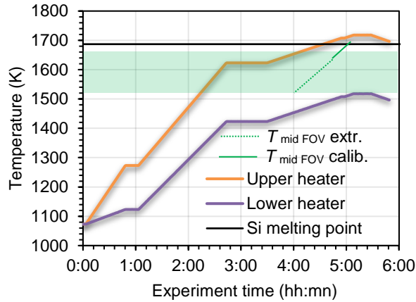
Figure 2: Temperature profiles of both heaters of the furnace and of the sample in the middle of the field of view (FOV, calibration and extrapolation). The black horizontal line corresponds to the Si melting isotherm. The temperature range within which the dislocation velocity measurements are carried out is highlighted with a green stripe.
