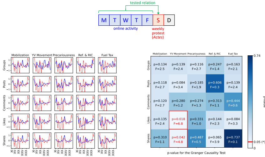
Fig. 11 The online predictors of the number of protesters: p-values of the Granger causality test between the levels of different types of online activity, and the time-series measuring the evolution of the number of protesters for Acte X .
