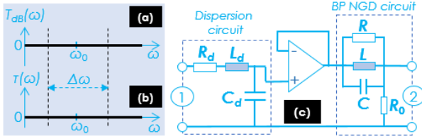
Fig. 3. Desired TF (a) magnitude and (b) GD specifications of (c) cascaded dispersion-NGD circuit.
