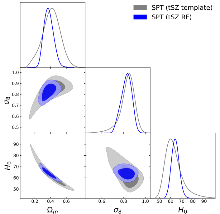
Fig. 3. Constraints on cosmological parameters obtained with SPT high- \ell data using the tSZ template as done in Reichardt et al. (2021, in grey) and using the tSZ power spectra derived from the halo model (in blue).
