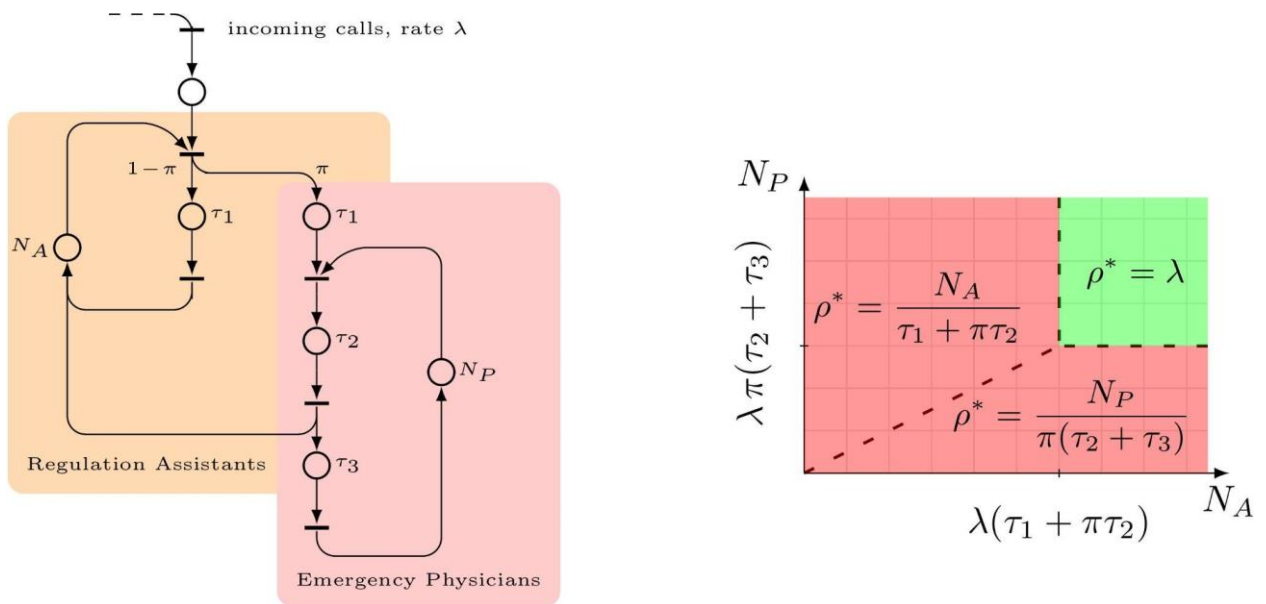
Fig. 2. Simplified Petri net representing a SAMU call centre, showing the chains of treatments by medical regulation assistants and emergency physicians (left); the throughput \rho as a function of the number of assistants N_A , of the number of physicians N_P , of the proportion of urgent calls \pi , of the conversation times \tau_i and of the input rate \lambda , following [3] – the congestion-free (sufficiently staffed) region is shown in green (right).
