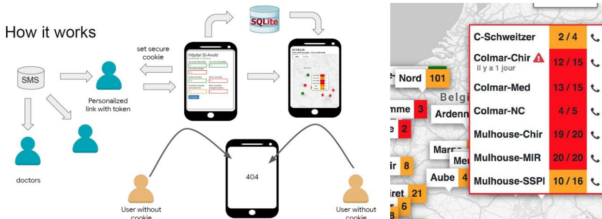
Fig. 1. Operation scheme of the ICUBAM app and its security protocol (left). Number of available beds over the total number of beds in each unit listed in the app (right). Lines colored in red indicate that more than 80% of beds are occupied, orange corresponds to 50-80% of occupied beds, and green corresponds to less than 50%.
