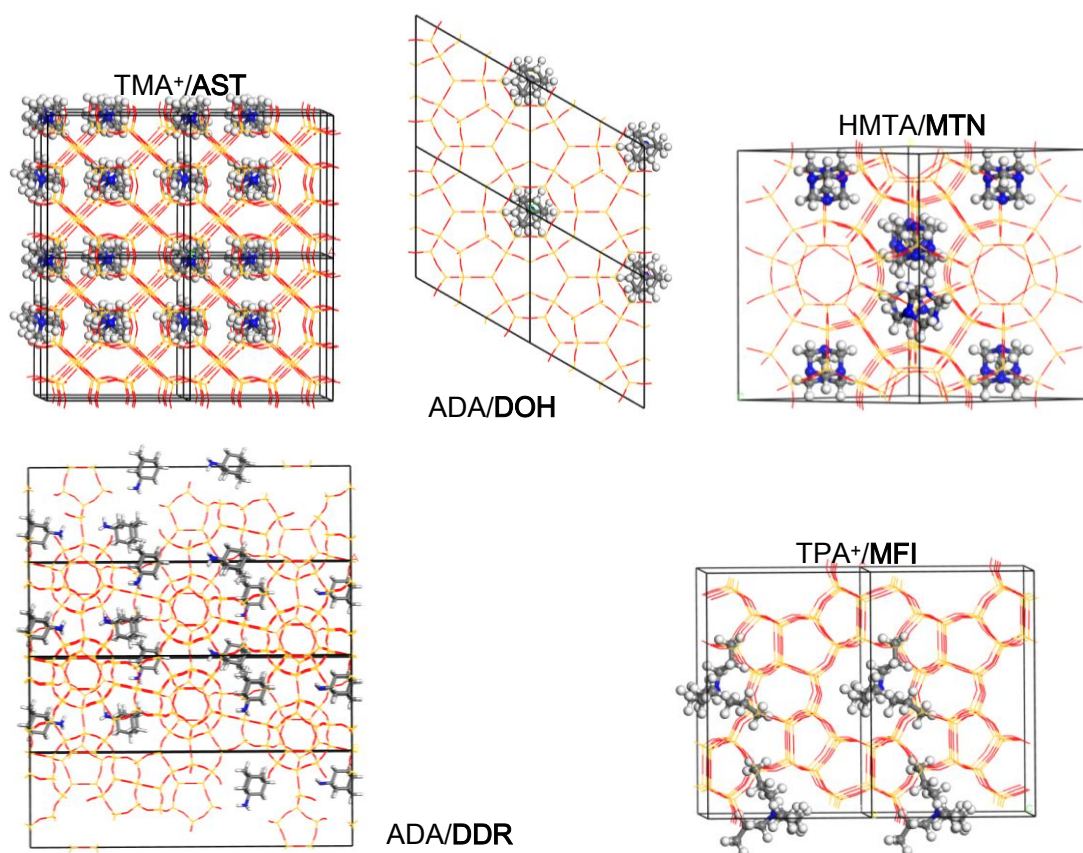
Figure 4. The occupancies and locations of respective SDA in the framework cuts, as found by simulated annealing: TMA + /AST; ADA/DOH; HMTA/MTN; ADA/DDR; TPA + /MFI.
