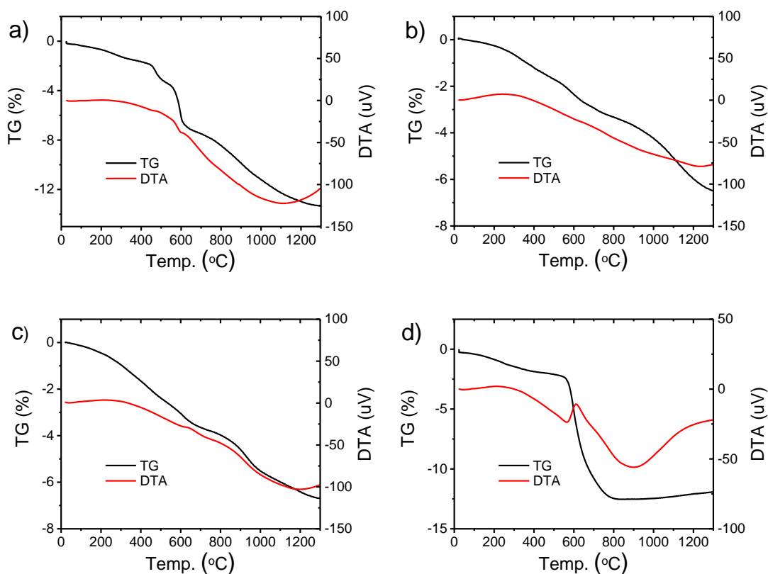
Figure 5. TG/DTA curves of the acidic medium synthesized SDA@SiO 2 clathrasils: a) TMA + /AST; b) ADA/DOH; c) HMTA/MTN; and d) ADA/DDR.
