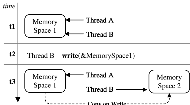
Fig. 10 Principle of the Copy-on-Write (CoW) mechanism.
