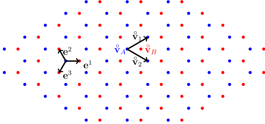
FIGURE 3. Bulk honeycomb structure, \mathbb{H} , comprised of A -site (blue) and B -site (red) triangular sublattices.
