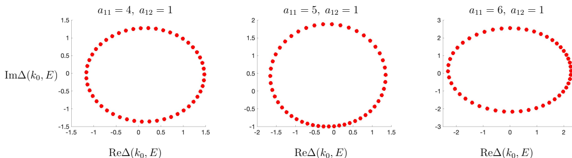
FIGURE 13. Plots of \Delta(k_0, E) in the complex plane when E takes the values specified in (7.22) with r_E = 0.01 and N_c = 50 .
