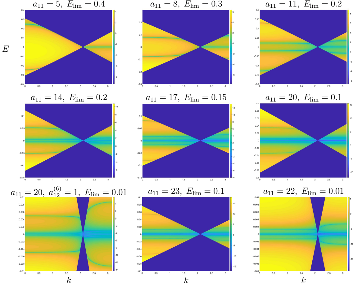
FIGURE 16. Plots of (k, E) \mapsto \log |\Delta(E, k)| for k \in (0, \pi) ( N_k = 600 points) and E \in (-E_{\text{lim}}, E_{\text{lim}}) ( N_E = 600 points) for various ordinary zigzag-like edges with a_{12} = 1 .
