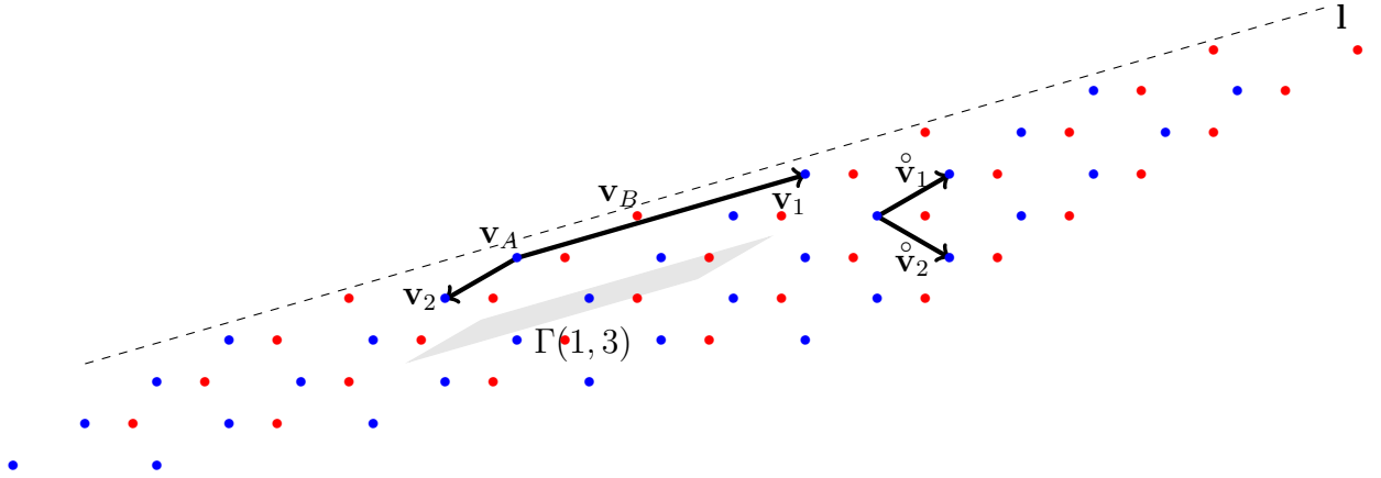
FIGURE 5. Notation for the edge defined by (a_{11}, a_{12}) = (3, 1) : the vectors \mathbf{v}_1 and \mathbf{v}_2 , the points \mathbf{v}_A and \mathbf{v}_B , and the parallelogram \Gamma(1, 3) .
