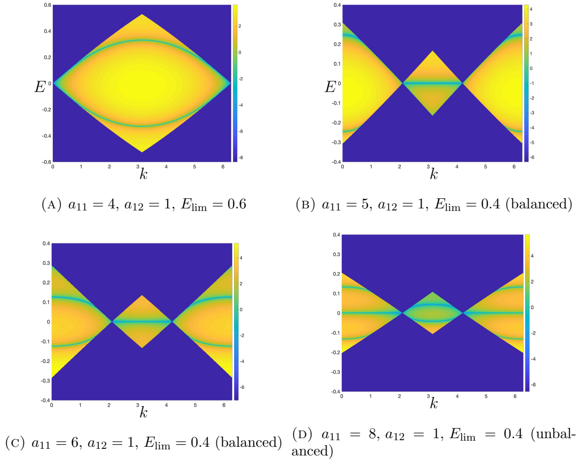
FIGURE 12. Plots of (k, E) \mapsto \log |\Delta(k, E)| for k \in (0, 2\pi) ( N_k = 1000 points) and E \in (-E_{\text{lim}}, E_{\text{lim}}) ( N_E = 1000 points), see (7.22). Note that the color scale is different from one figure to another.
