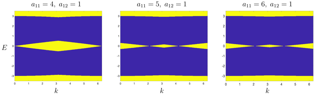
FIGURE 8. For each k \in [0, 2\pi] , we indicate in blue (resp. in yellow) the essential spectrum (resp. the resolvent set or the gaps) of H_{\text{bulk}}(k) in the interval E \in (-3.5, 3.5) .
