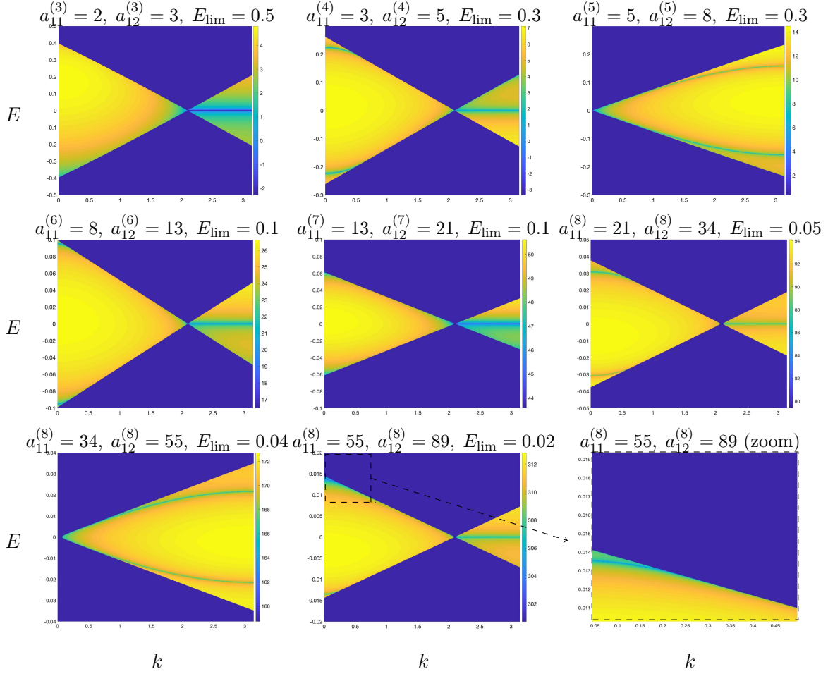
FIGURE 17. Plots of (k, E) \mapsto \log |\Delta(k, E)| for k \in (0, \pi) ( N_k = 1000 points) and E \in (-E_{\text{lim}}, E_{\text{lim}}) ( N_E = 1000 points) and with n_{\text{min}}^A = n_{\text{min}}^B = 0 for the Fibonacci sequence.
