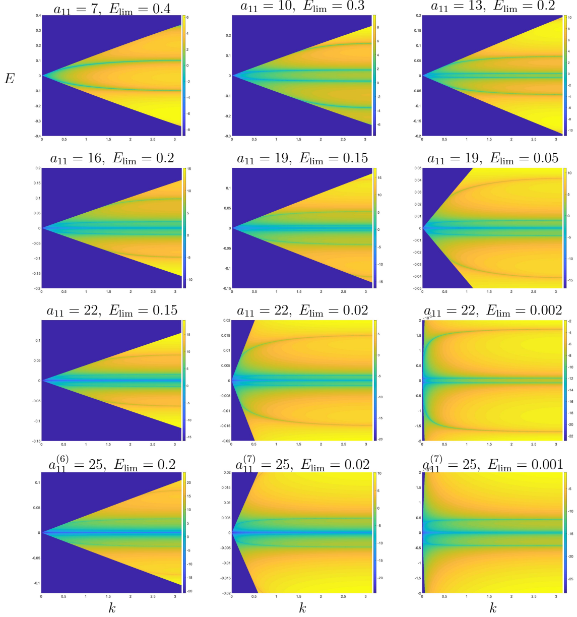
FIGURE 15. Plots of (k, E) \mapsto \log |\Delta(E, k)| for k \in (0, \pi) ( N_k = 1000 points) and E \in (-E_{\text{lim}}, E_{\text{lim}}) ( N_E = 1000 points) for various armchair-like edges with a_{12} = 1 .
