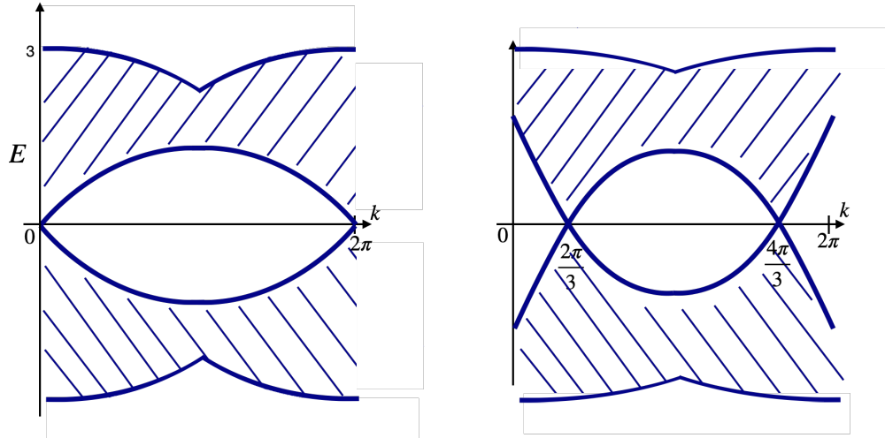
FIGURE 7. Shaded regions indicate essential spectrum of H_{\text{bulk}}(k) and H_{\sharp}(k) for different types of rational edges; armchair type edge (left) and zigzag type edge (right).
