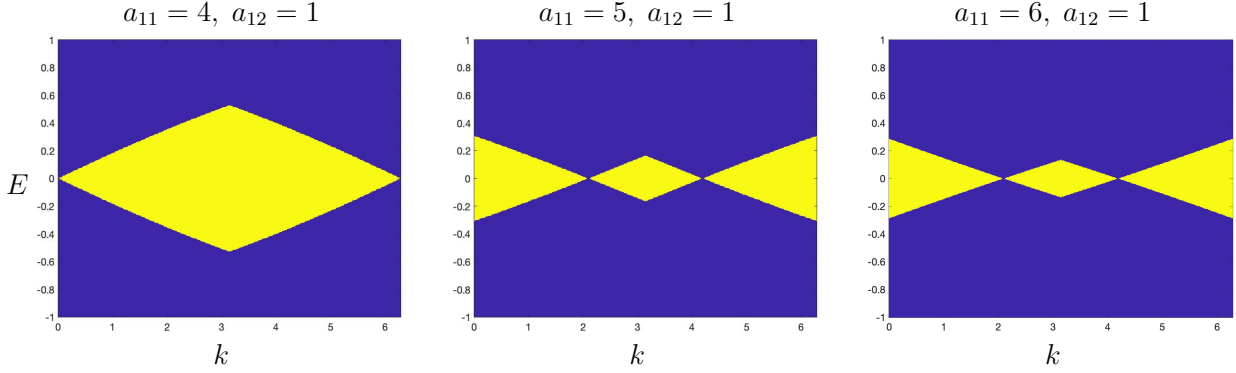
FIGURE 9. For each k \in [0, 2\pi] , we indicate in blue (resp. in yellow) the essential spectrum (resp. the resolvent set or the gaps) of H_{\text{bulk}}(k) in the interval E \in (-1, 1) .
