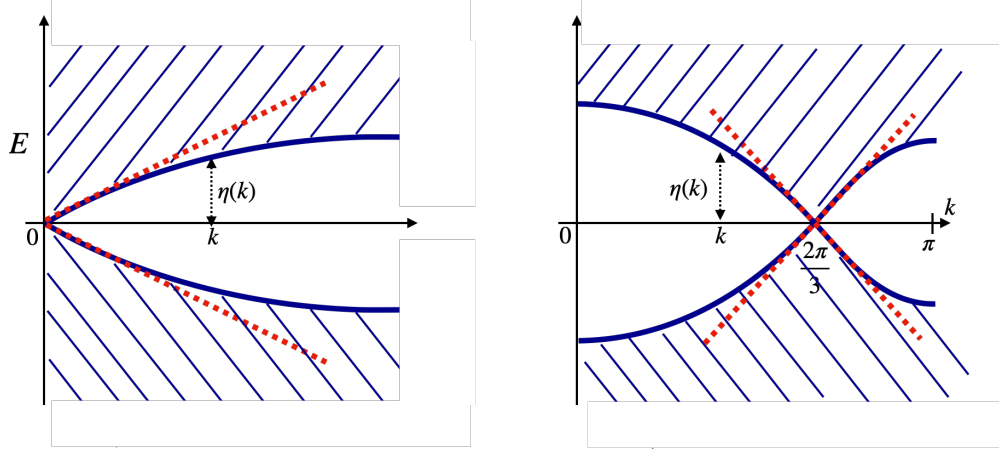
FIGURE 10. Schematic for Edge of the Wedge Proposition 3.6. Blue regions are essential spectrum and red dotted lines have slopes of magnitude \alpha = \frac{\sqrt{3}}{2} |\mathbf{v}_1|^{-1} = \frac{\sqrt{3}}{2} (a_{11}^2 + a_{11}a_{12} + a_{12}^2)^{-1/2} : armchair type edge (left) and zigzag type edge (right).
