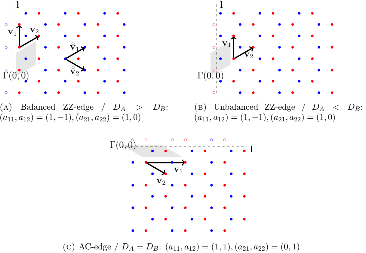
FIGURE 6. \mathbb{H}_\sharp for the classical ZZ and AC edges, balanced and unbalanced; see Definition 2.3. A - sites are in blue and B - sites are in red. The edge, \mathbf{l} , is indicated with a dashed line. The parallelogram \Gamma(0, 0) is shaded gray; see Remark 2.4.
