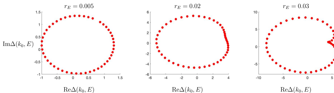
FIGURE 14. For the edge a_{11} = 6 , a_{12} = 1 , plots of \Delta(k_0, E) in the complex plane when E takes the values specified in (7.22) with N_c = 50 and various values of r_E .
