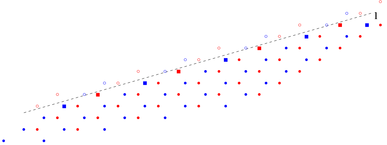
FIGURE 4. The edge defined by (a_{11}, a_{12}) = (3, 1) . A - and B - sublattice vertices of \mathbb{H}_\sharp are indicated by colored circles and colored squares. Colored squares indicate the frontier sites, as defined in the introduction. Empty circles indicate vertices outside \mathbb{H}_\sharp , which are nearest neighbors to vertices in \mathbb{H}_\sharp .
