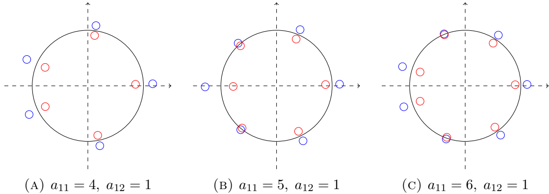
FIGURE 11. The roots of the polynomial P_{E,k}(\zeta) for E = 0.1 and k = 3 for three different edges
