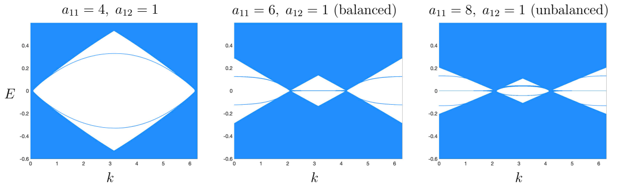
FIGURE 2. l_k^2 spectrum of H_{\#,k} versus k for several choices of edges: (i) (a_{11}, a_{12}) = (4, 1) , an AC-type edge, (ii) (a_{11}, a_{12}) = (6, 1) , a ZZ-type balanced edge and (iii) (a_{11}, a_{12}) = (8, 1) , a ZZ-type unbalanced edge.
