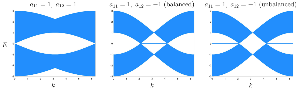
FIGURE 1. l_k^2 spectrum of H_{\#,k} versus k for several choices of edges: (i) (a_{11}, a_{12}) = (1, 1) , the classical armchair edge, (ii) (a_{11}, a_{12}) = (1, -1) , the classical zigzag balanced (aka ordinary) edge, (iii) (a_{11}, a_{12}) = (1, -1) , the classical zigzag unbalanced (aka bearded) edge.
