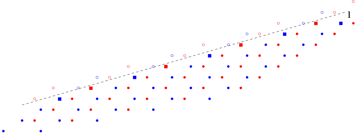
FIGURE 4. The edge defined by (a_{11}, a_{12}) = (3, 1) . A - and B - sublattice vertices of \mathbb{H}_\sharp are indicated by colored circles and colored squares. Colored squares indicate the frontier sites, as defined in the introduction. Empty circles indicate vertices outside \mathbb{H}_\sharp , which are nearest neighbors to vertices in \mathbb{H}_\sharp .
