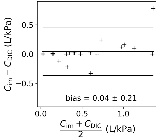
Figure 5: Bland–Altman plot to compare the image and displacement criteria. The quantities used for the comparison are the compliances computed by both criteria. C_{\text{DIC}} and C_{\text{im}} are the compliances estimated with the displacement criterion and the image criterion, respectively.
