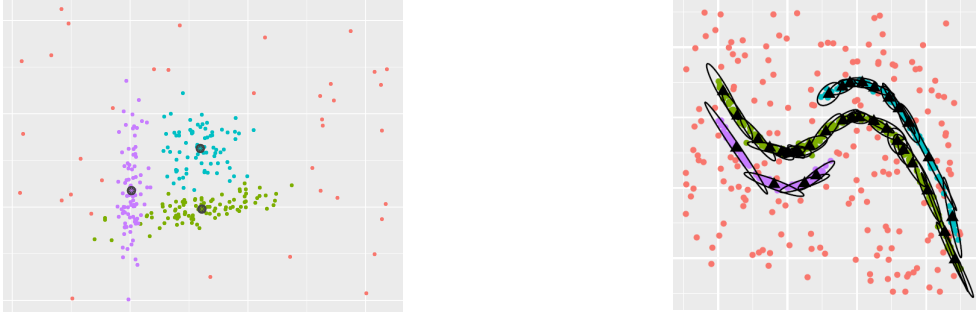
FIGURE 4. Data clustering with a straight use of the criterion \gamma_{\mathbb{X},h}(\hat{\mathbf{t}}, \cdot) (left), with a hierarchical type clustering based on \gamma_{\mathbb{X},h}(\hat{\mathbf{t}}, \cdot) (right)
