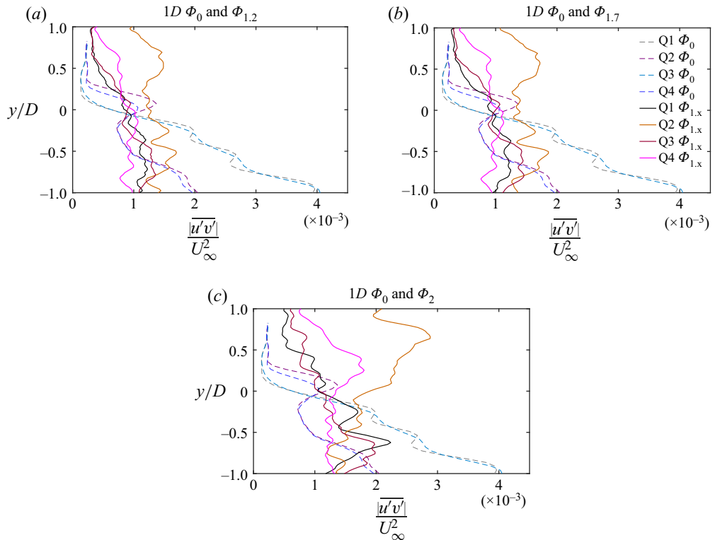
Figure 18. Vertical profiles of quadrant analysis at wake location 1D . Dashed lines represent each quadrant for the single-phase flow case ( \Phi_0 ), while solid lines represent each quadrant for \Phi_{1.2} (a), \Phi_{1.7} (b) and \Phi_2 (c) which represent two-phase flow with water flow rates of 1.2, 1.7 and 21 \text{ min}^{-1} and volume fractions of 7.11 \times 10^{-6} , 10.3 \times 10^{-6} and 12.3 \times 10^{-6} , respectively. Flow direction is from the left, and y/D = 0 is the centre of the disk.
