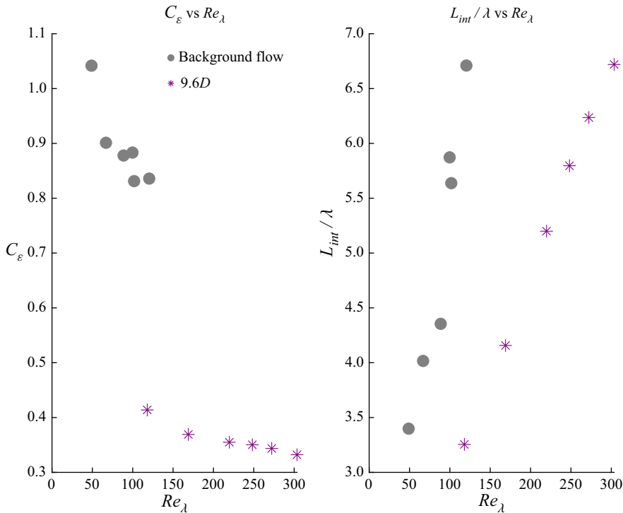
Figure 11. Values of C_\varepsilon and L_{int}/\lambda are plotted vs the Taylor scale Reynolds number Re_\lambda for the background flow and the wake at 9.6D at tunnel speeds U_\infty = 1.3, 4.9, 8.3, 10.6, 12.0 and 15.8 \text{ m s}^{-1} .
