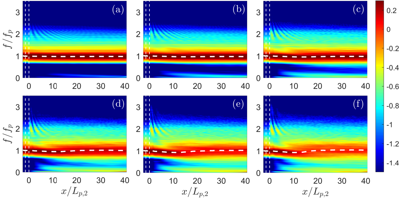
Figure 8: Evolution of the normalized wave spectra in cases 2–7, shown in panels (a–f) correspondingly. \log_{10}(S(f)f_p/m_0) is plotted in the colormap with a logarithmic scale. The close-to-horizontal dash line represents the evolution of \hat{f}_p and the vertical dash lines outline the extent of the bottom slope.
