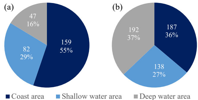
Figure 1: Statistics of the freak waves reported in mass media over the period 2006 – 2018, based on the works of Nikolkina and Didenkulova (2011b) and Didenkulova and Pelinovsky (2020). The number and percentage of freak wave events are shown in (a), and the loss of lives in (b).
