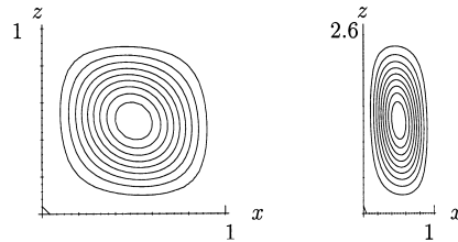
Fig. 9. Streamlines of the variational solution at Ra_{cE} when A = 1 (left) and A = 2.6 (right) and Le = 11 , Pr = 1 . In both cases the flow is clockwise.
