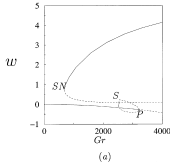
Fig. 13. (a) The vertical velocity w(0.388, 0.5) in a square container with N = -1.01 as a function of the Grashof number Gr . (b) Enlargement of (a). The resolution is 15 \times 15 . Stable (unstable) solutions are indicated by continuous (dashed) lines. Positive w implies clockwise circulation.
