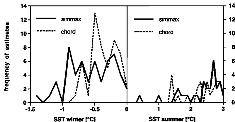
Figure 9. Comparison of the SST estimates at the cold end generated by modern analog technique (MAT) with squared chord distance dissimilarity index and by the SIMMAX distance-weighted version.
