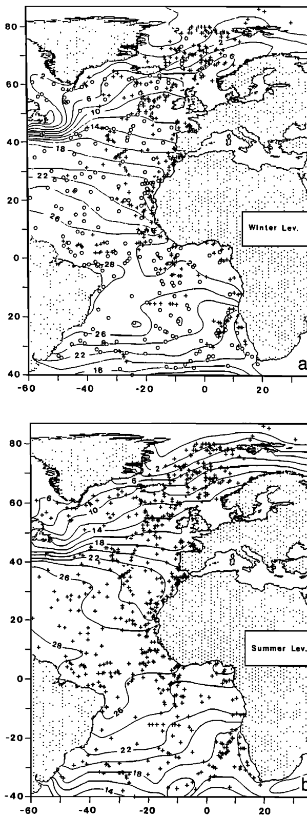
Figure 1. Location of 738 sediment surface samples used for the SIMMAX technique and sea surface temperature (SST) of Levitus [1982], derived from the original 1x1° grid: (a) northern hemisphere winter; (b) northern hemisphere summer. Circles mark SPECMAP data.
