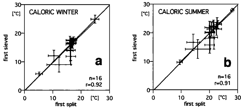
Figure 3. Comparison of the SST estimates based on 16 samples counted twice. The x-axis shows estimates of samples which had been split first, then sieved; the y-axis shows estimates from samples which had been sieved first and then split: (a) caloric winter; (b) caloric summer. The error bars indicate the standard deviation of the 10 most similar analogs.
