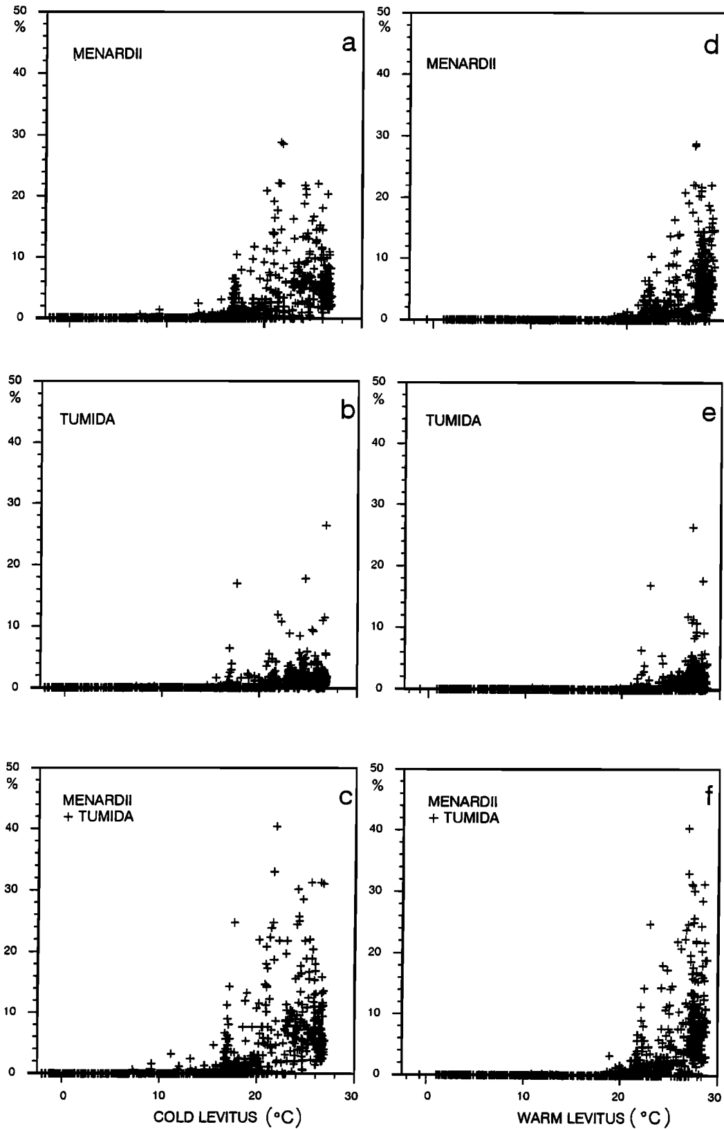
Figure 5. Sea surface temperature preference of the menardiform globorotalias: caloric winter SST ( x -axis in degrees Celsius) versus (a) G. menardii , (b) G. tumida , (c) G. menardii plus tumida ; caloric summer SST ( x -axis in degrees Celsius) versus (d) G. menardii , (e) G. tumida , (f) G. menardii +plus tumida ( y -axis in percentages of total planktonic foraminifera).
