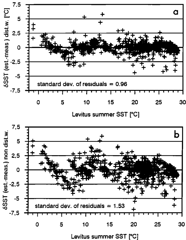
Figure 8. Deviation of SIMMAX versus Levitus [1982] summer temperatures: (a) distance-weighted estimates; (b) non-distance-weighted estimates.
