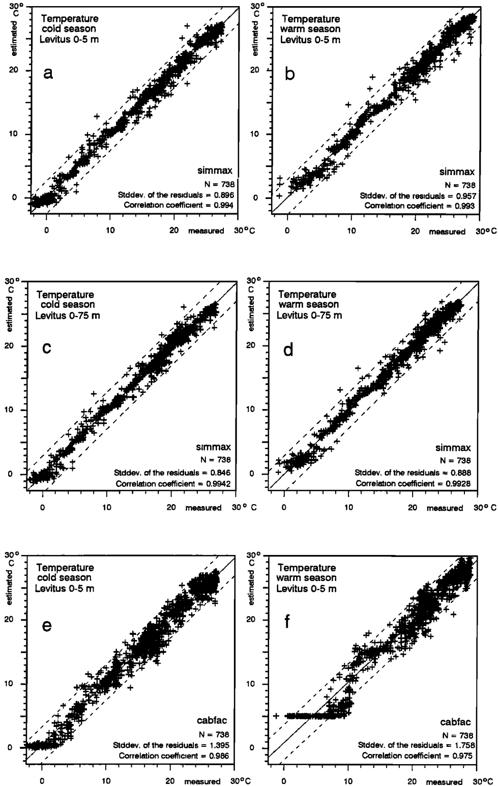
Figure 6. Comparison between SIMMAX estimated and measured SST at 0 m (level 1); \pm 2^\circ\text{C} deviation is indicated for (a) caloric winter, and (b) caloric summer (x and y -axis in degrees Celsius). Comparison between SIMMAX estimated and Levitus measured SST for 0- to 75-m depth, the level showing the best fit for (c) caloric winter and (d) caloric summer. Hatched lines indicate the \pm 2^\circ\text{C} deviation. Comparison between Climate: Long-Range Investigation, Mapping, and Prediction (CLIMAP) transfer technique-estimated and Levitus [1982] measured temperatures for 0-m (level 1): (e) caloric winter, f) caloric summer. Hatched lines indicate the \pm 2^\circ\text{C} deviation.
