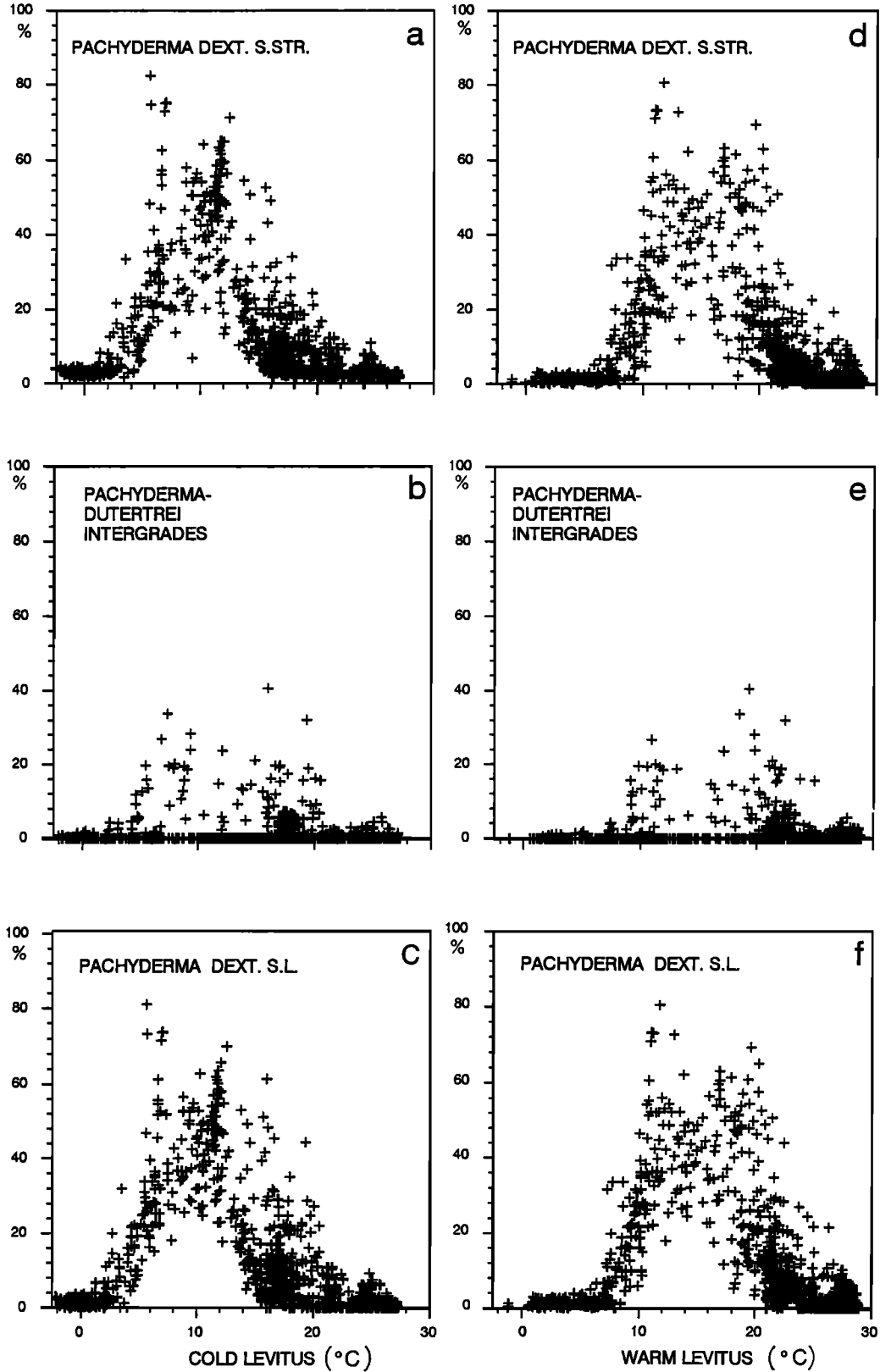
Figure 4. Sea surface temperature preference (x-axis in degrees Celsius) of Neogloboquadrina pachyderma var. dextra s. str. , the intergrades between N. dutertrei and pachyderma , and the lumped N. pachyderma var. dextra s. l. : (a-c) caloric winter temperatures; (d-f) caloric summer temperatures (y-axis is the percentages of total planktonic foraminifera).
