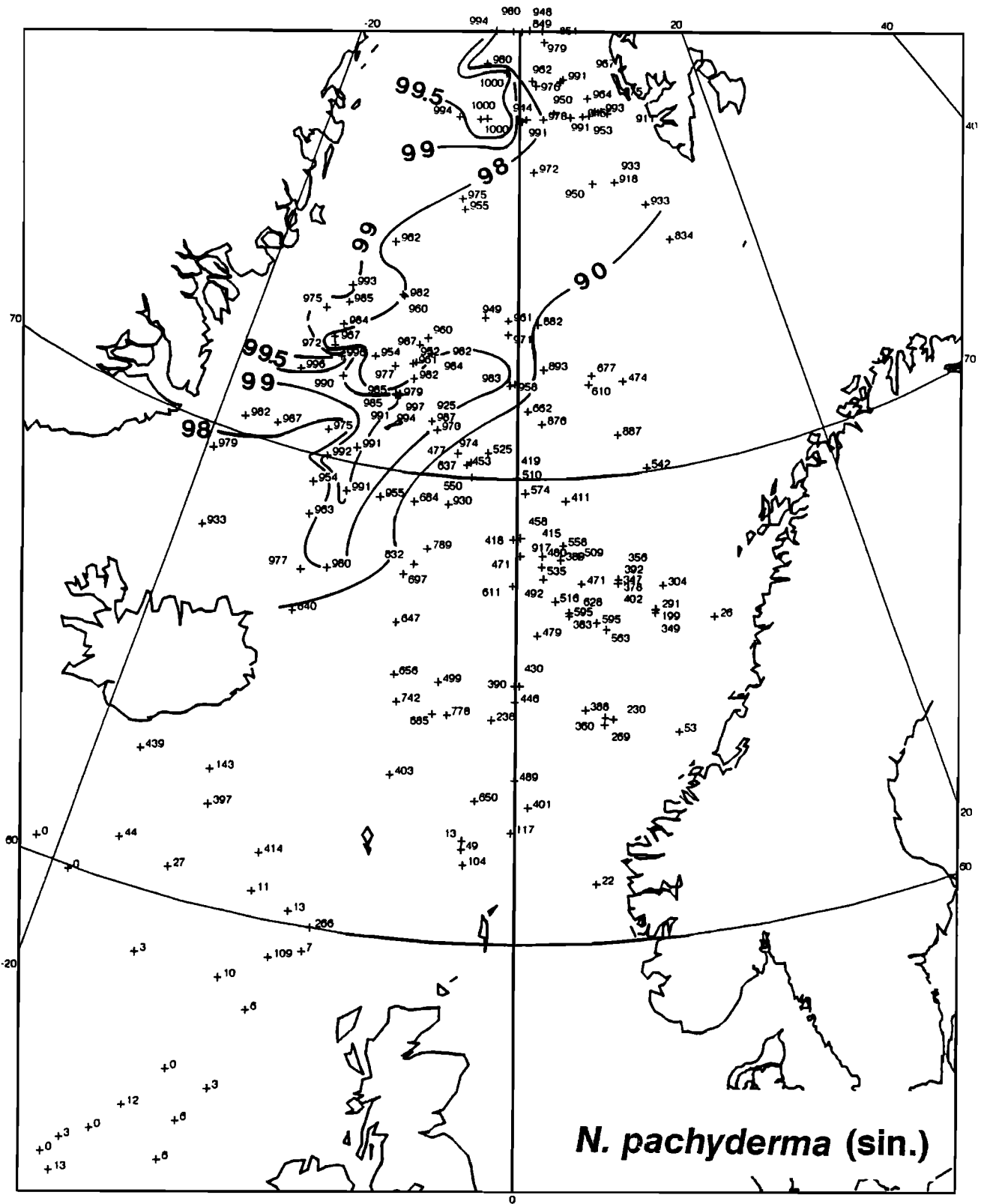
Figure 2. Areal distribution of the percentages of left-coiling N. pachyderma in total planktonic foraminifera of the pelagic sediments in the Norwegian-Greenland Sea. Isolines fitted by eye. (Small numbers at the stations in percent x 0.1).
