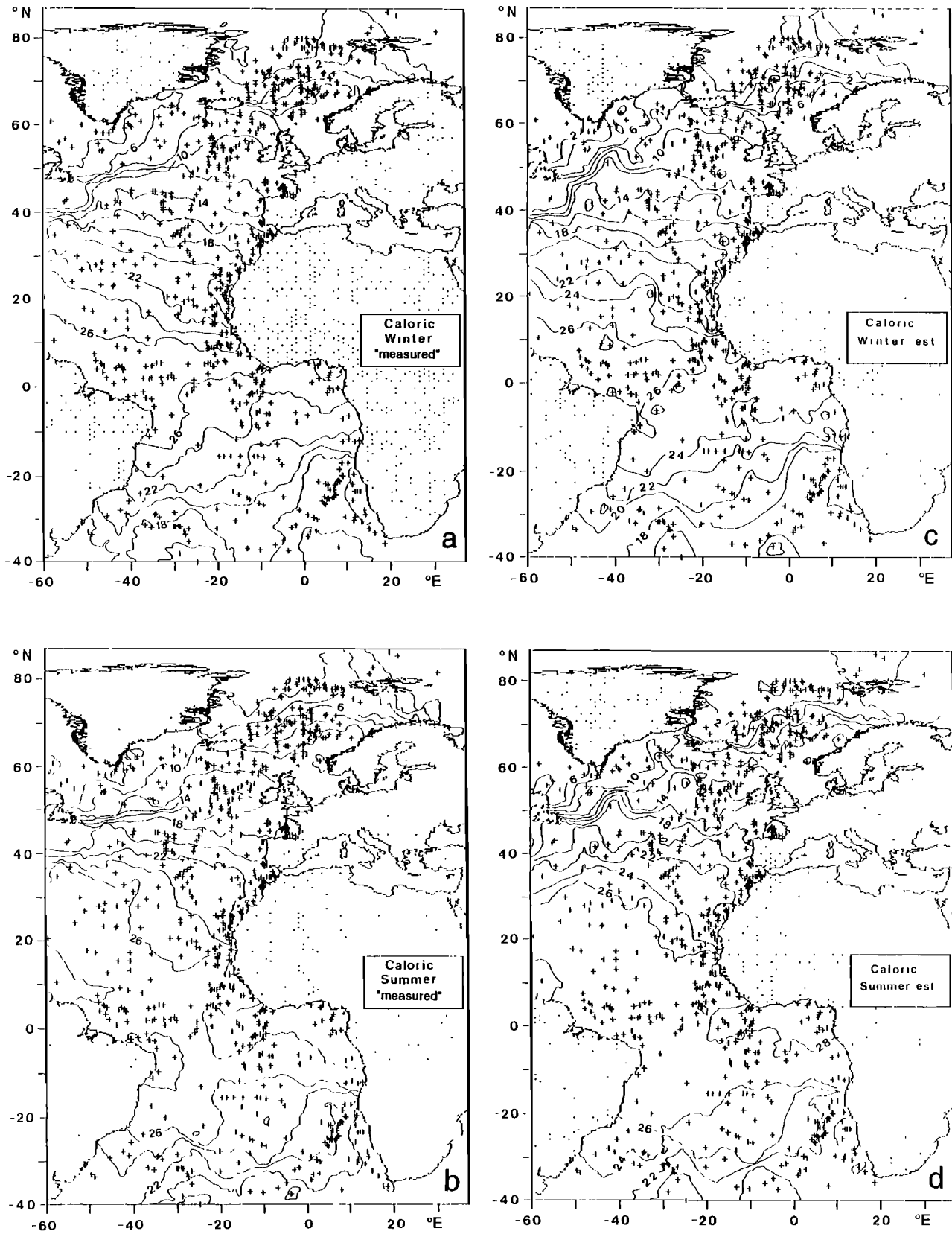
Figure 7. Areal distribution of SST in the Atlantic, derived only by the calibration data: (a) caloric winter SST interpolated from Levitus [1982]; (b) caloric summer SST interpolated from Levitus [1982]; (c) caloric winter SST estimated by SIMMAX; (d) caloric summer SST estimated by SIMMAX.
