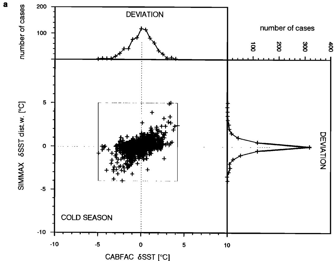
Figure 10. Comparison of SST deviations (in degrees Celsius) from Levitus [1982] data set, as derived from SIMMAX and CLIMAP transfer technique (model 738-8-26) at 0-m water depth: (a) caloric winter; (b) caloric summer. Frequency distribution of SIMMAX deviation values is clearly more focussed to zero than the distribution of CLIMAP transfer technique values.
