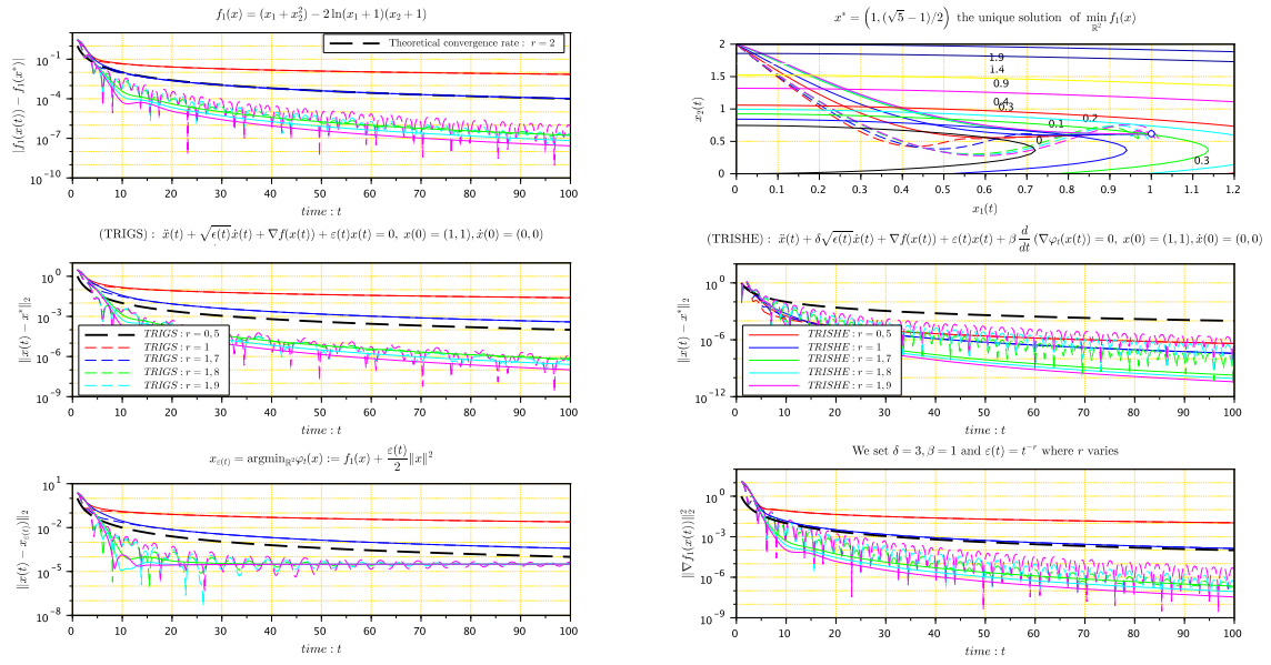
Fig. 1 Convergence rates of values f_1(x(t)) - f_1(x^*) , of trajectories \|x(t) - x^*\|_2 , and gradients \|\nabla f_1(x(t))\|_2 .
