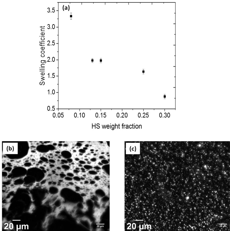
Figure S 2. a) Swelling coefficient diagram of the TPU P3000-MDI-BDO as a function of hard segment (HS) content; b) Fluorescence microscopy images of the bitumen-TPU blend made with a TPU at low HS content (8 wt%); c) Fluorescence microscopy images of the bitumen-TPU blend made with a TPU at high HS content (30 wt%).
