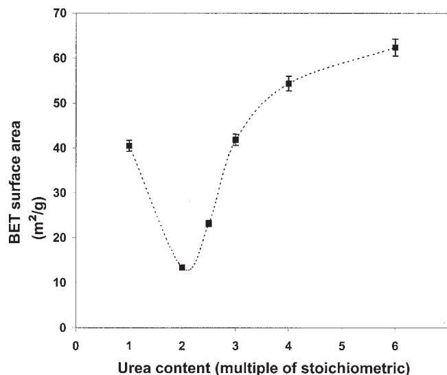
Fig. 2. Variation of BET surface area ( \text{m}^2/\text{g} ) for \text{Mg}_{0.8}\text{Co}_{0.2}\text{O} with fuel content.
