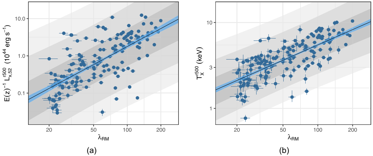
Figure 10. Luminosity–richness (a) and temperature–richness (b) relation of the SDSSRM–XCS _{T_X, \text{vol}} . For each relation, the best fit to the data (see Section 4.2) is represented by the blue solid line, and the light blue shaded region represents the 68 per cent confidence interval of the mean logarithmic relation. The grey bands represent the 1\sigma , 2\sigma , and 3\sigma intrinsic scatter.
