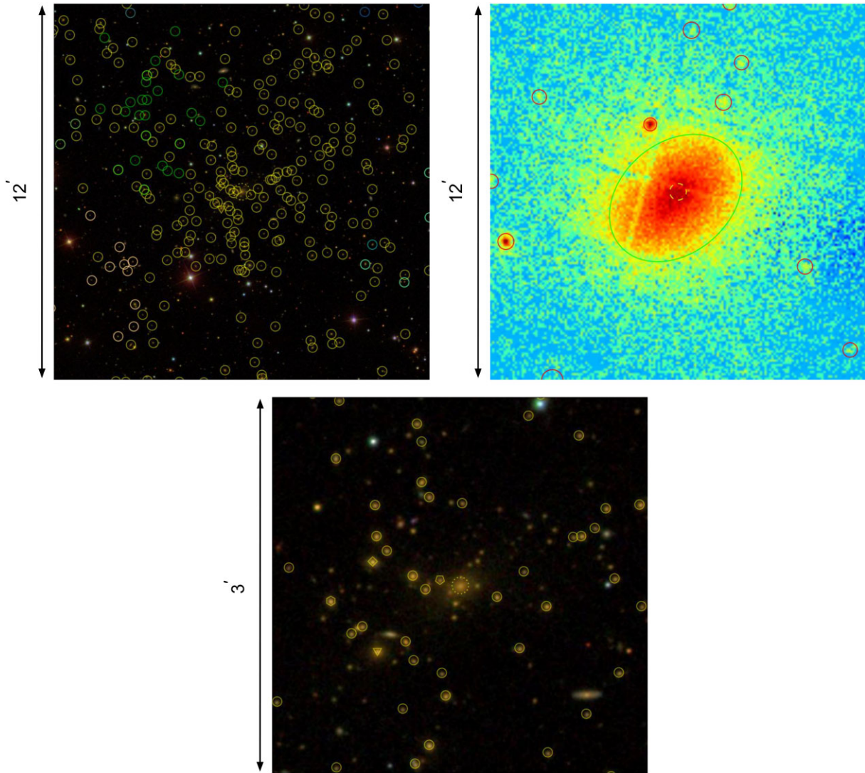
Figure 2. An example of a cluster in the SDSSRM–XMM ext sample (Table 1). Top left: SDSS optical image of the cluster XMMXCS J164020.2+464227.1 ( SDSS RMID = 2), commonly referred to as Abell 2219, at a redshift of z = 0.23 and richness of \lambda_{\text{RM}} = 199 . The dashed yellow circle and the other solid yellow shapes highlight the galaxies associated RMID = 2. Galaxy members of other nearby RM clusters nearby are circled in different colours (e.g. green, turquoise, and cream); Top right: XMM X-ray observation of the matched XCS extended source. Green (red) regions highlight extended (point) XAPA sources detected in the observation. Bottom middle: A zoom into the SDSS optical image. The yellow circle (dashed), triangle, diamond, pentagon, and hexagon represent, respectively, the 1st, 2nd, 3rd, 4th, and 5th most probable, according to the RM algorithm, candidate for the central galaxy.
