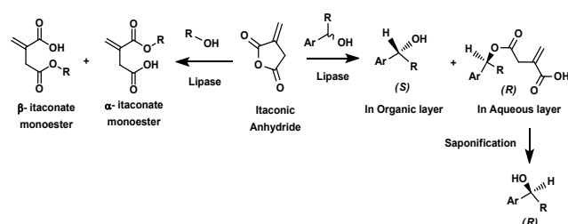
Scheme 1: Process Opening IAn with a series of primary and secondary achiral and chiral alcohols.
