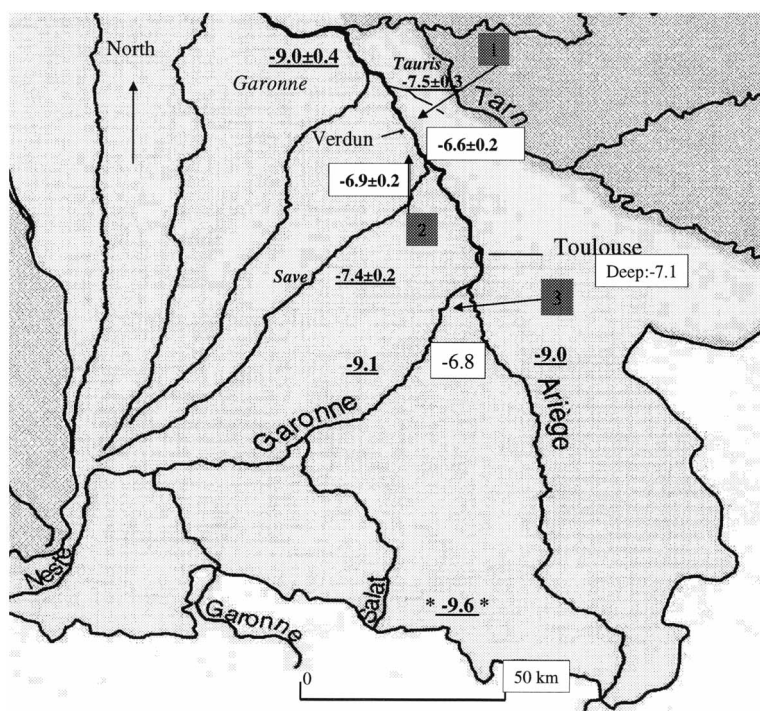
FIGURE 1 Typical \delta^{18}\text{O} values of water in the Garonne valley, in the south-west of France, near Toulouse. The values of the surface water are underlined; the “*” indicates a snow sample; white rectangles indicate ground water values; the one at Toulouse corresponds to deep ground water (53 m deep below surface). The numbers in grey rectangles indicate the place of the reference wells for the ground water: 1 is Monbéqui, 2 is St Pierre and 3 is Pinsaguel (confluence).
