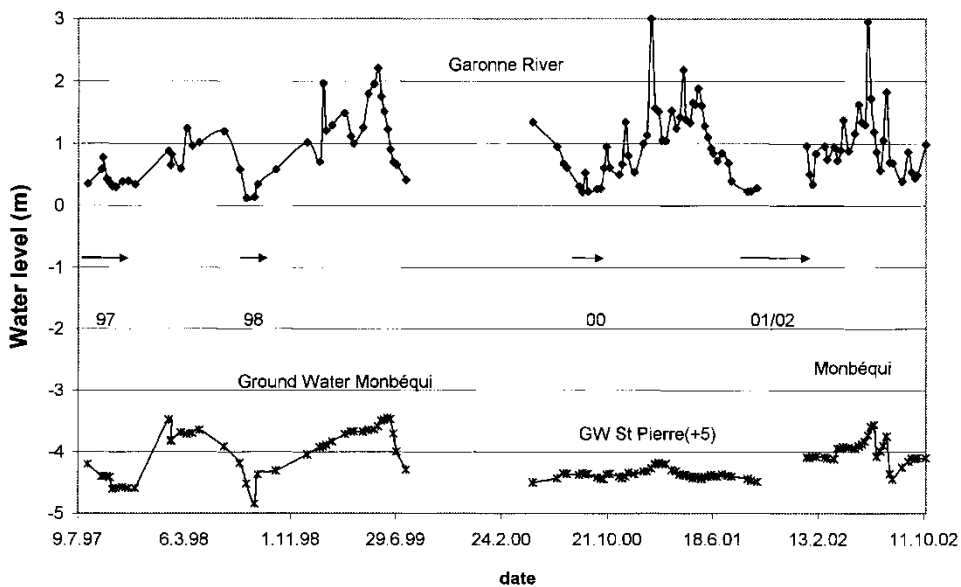
FIGURE 4 Level of the Garonne River at Verdun for the sampling dates during the study time and comparison with the ground water level in Monbéqui and St. Pierre. The St. Pierre values have been upgraded by 5 m for a better comparison of the variations. The arrows indicate the low water period for the year with the corresponding date.
