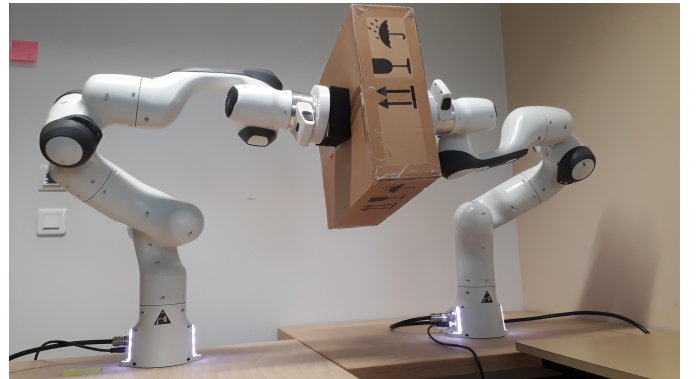
Fig. 2: Two Panda manipulators with soft, deformable pads attached to the end-effectors. We initiate contacts for swift box grabbing with pre-impact velocities of 0.61 m/s. The video is available at: https://youtu.be/dPLN87knF8
