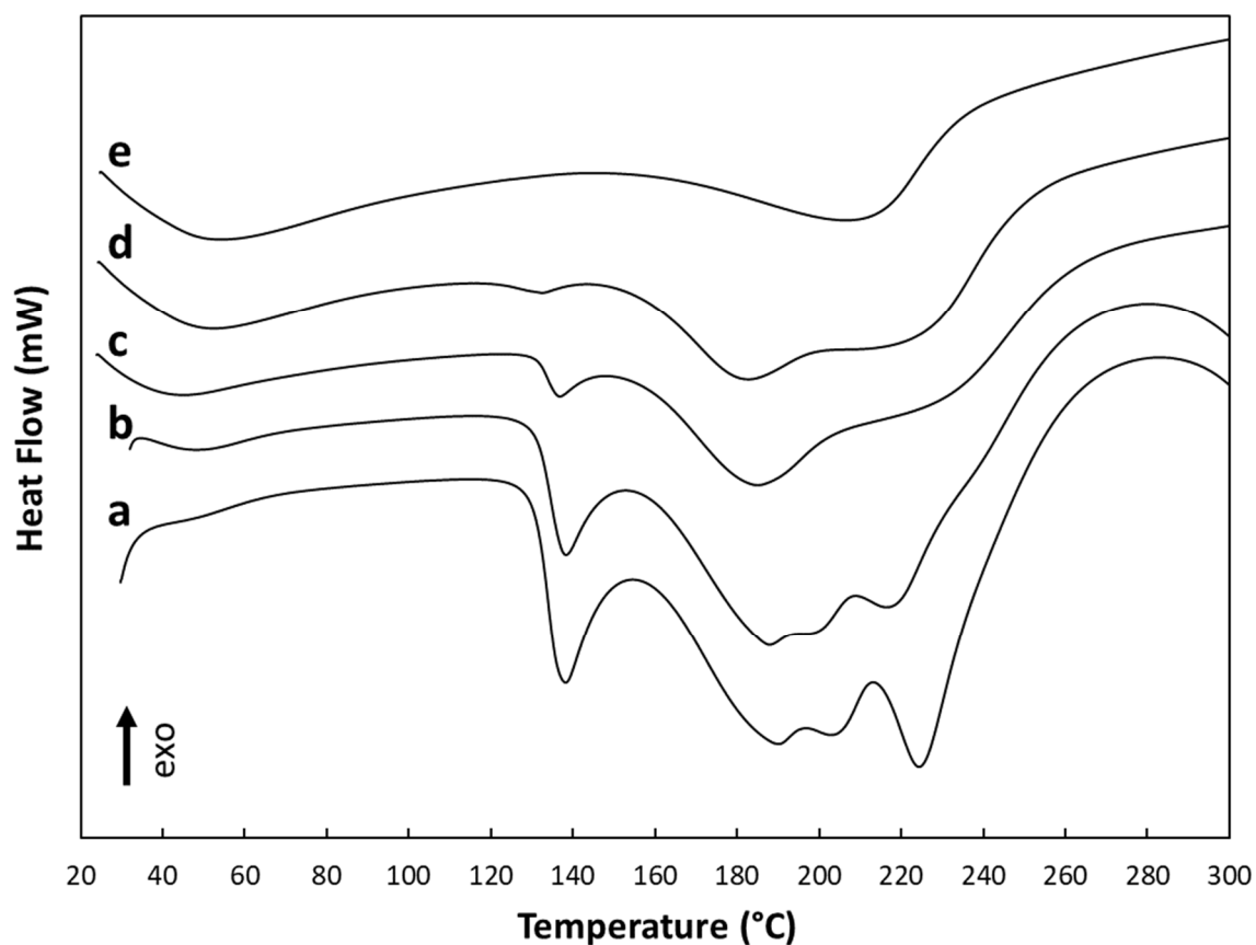
Fig. 5. DSC curves of (a) kaolin ground for 1 h with 66 m% urea (b) sample (a) washed three times with isopropanol, (c) sample (a) washed seven times with isopropanol, (d) kaolin ground for 2 h with 25 m% urea and (e) sample (d) washed three times with isopropanol.
