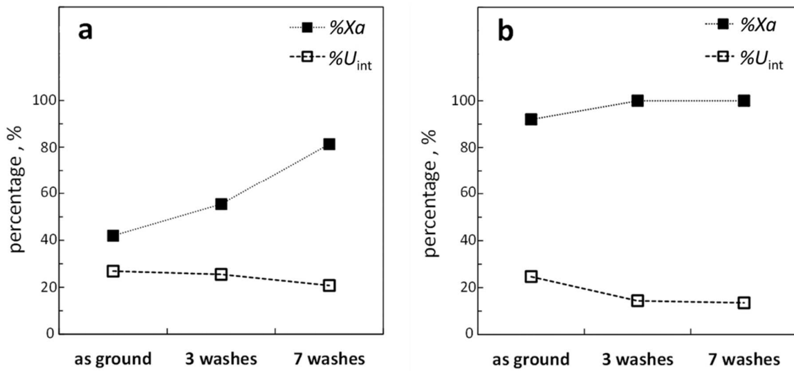
Fig.6. Effect of isopropanol washes on the amount of intercalated urea relative to total urea ( \%X_a ) or relative to the kaolin-urea content ( \%U_{int} ) for (a) kaolin ground with 66 m% urea for 1 h and (b) kaolin ground with 25 m% urea for 2 h. The error bars (the average deviation from the mean of duplicate measurements) are smaller than the size of the symbols.
