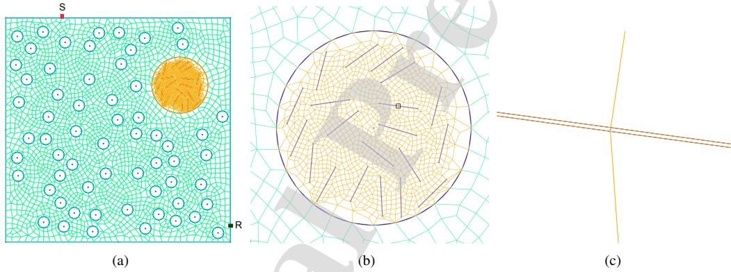
Figure 2: An example mesh for a heterogeneous model with 20 cracks of random orientations. Each crack is modeled by one void cell, and the size of the cracks is 10 mm × 0.01 mm. The blue lines represent the contour of the matrix, the EDZ, and the cracks. The matrix size is 200 mm × 200 mm, and the circular EDZ center is located at (155 mm, 140 mm). The source position is (50 mm, 200 mm). (a) Mesh of the global configuration; (b) Magnified view of the meshed EDZ; (c) Magnified view of one crack corresponding to the square in (b).
