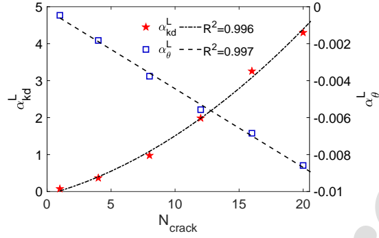
Figure 5: Slopes of CWI observables with crack length changes versus crack density N_{crack} . For each fixed number of random cracks ( N_{crack} \in [1, 4, 8, 12, 16, 20] ), five numerical models were used. For each group of models, five crack disorder arrangements were considered in order to calculate the mean value of \alpha_{Kd}^L (red pentagram) and \alpha_{\theta}^L (blue square), their slopes versus crack density N_{crack} are obtained with linear and quadratic regression and illustrated with dash-dot line and dashed line, respectively.
