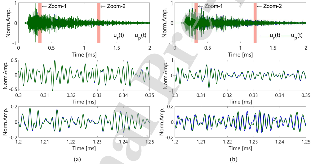
Figure 3: Examples of temporal signals for the model with (a) four random cracks and (b) 20 random cracks. The blue lines correspond to the reference model with no change in the crack length ( \Delta L_{crack}/L_{crack} = 0 ), whereas the green lines correspond to the model with an effective change in crack lengths ( \Delta L_{crack}/L_{crack} = +1.6\% ), assumed to originate from the pump wave action.
