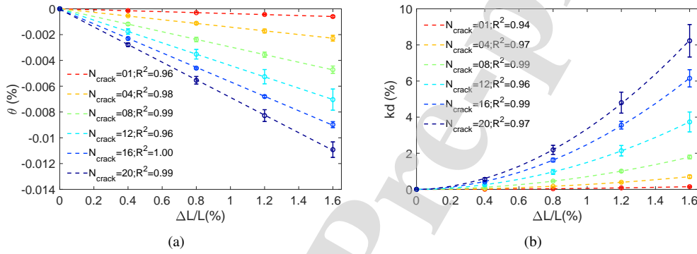
Figure 6: CWI observables versus changes in crack length ( \Delta L_{crack}/L_{crack} ) for the reverberating medium. For each fixed number of random cracks ( N_{crack} \in [1, 4, 8, 12, 16, 20] ), six numerical models were used: (a) Relative variation in velocity \theta_{coda} versus \Delta L_{crack}/L_{crack} ; (b) Remnant decorrelation coefficient Kd versus \Delta L_{crack}/L_{crack} .
