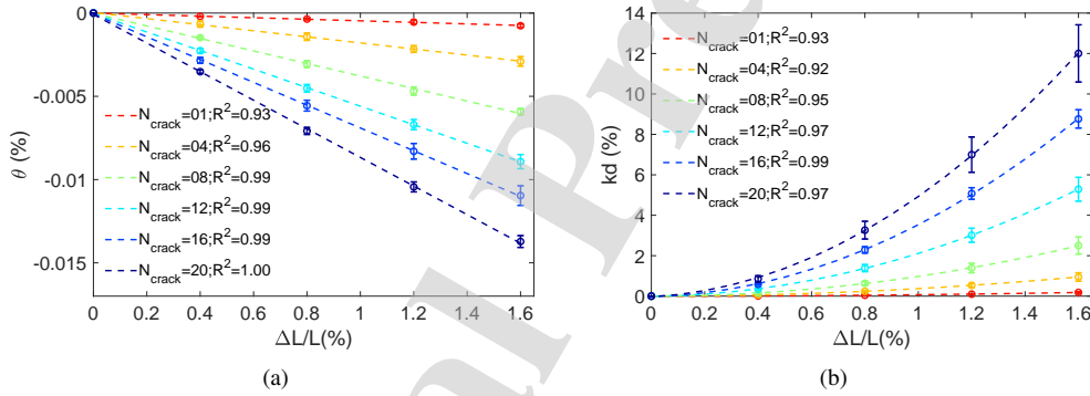
Figure 4: CWI observables versus changes in the crack length ( \Delta L_{crack}/L_{crack} ). For each fixed number of random cracks ( N_{crack} \in [1, 4, 8, 12, 16, 20] ), five numerical models were used. (a) Relative variation in velocity \theta_{coda} versus \Delta L_{crack}/L_{crack} ; (b) Remnant decorrelation coefficient Kd versus \Delta L_{crack}/L_{crack} .
