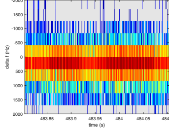
SG Spectrogram
