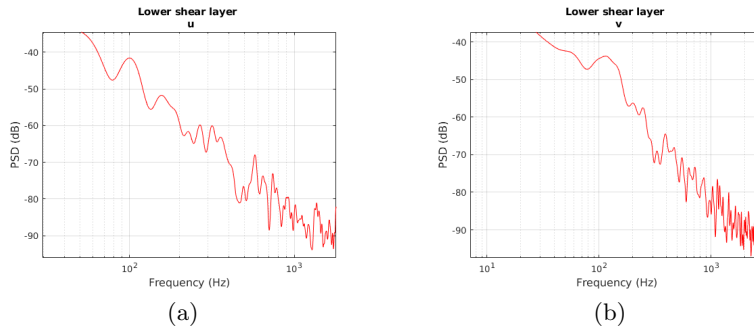
Fig. 5: PSD of monitor point in the shear layer. (a) and (b) correspond to the position ( x/c = 1.14 , y/c = -0.20 )
