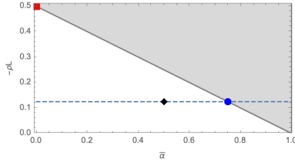
Figure 2: The grey region indicates where convergence provably cannot be guaranteed by Theorem 3.4 . The dashed line indicates where \rho = -1/8L . This is the condition under which ( Diakonikolas et al., 2021, Thm. 3.2 ) shows the first convergence result ( \blacklozenge ). Corollary 3.2 improves their result by matching the lower bound for any \bar{\alpha} , in particular for \bar{\alpha} = 3/4 ( \bullet ). The adaptive scheme in Theorem 3.1 matches the smallest possible \rho for any (EG+) scheme with fixed stepsize ( \blacksquare ).
