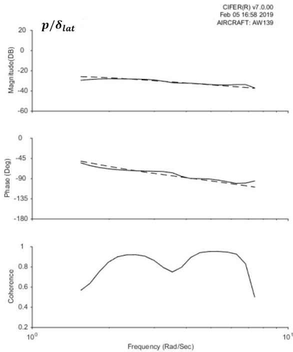
Figure 5. Lateral-directional frequency response – roll rate to lateral stick
