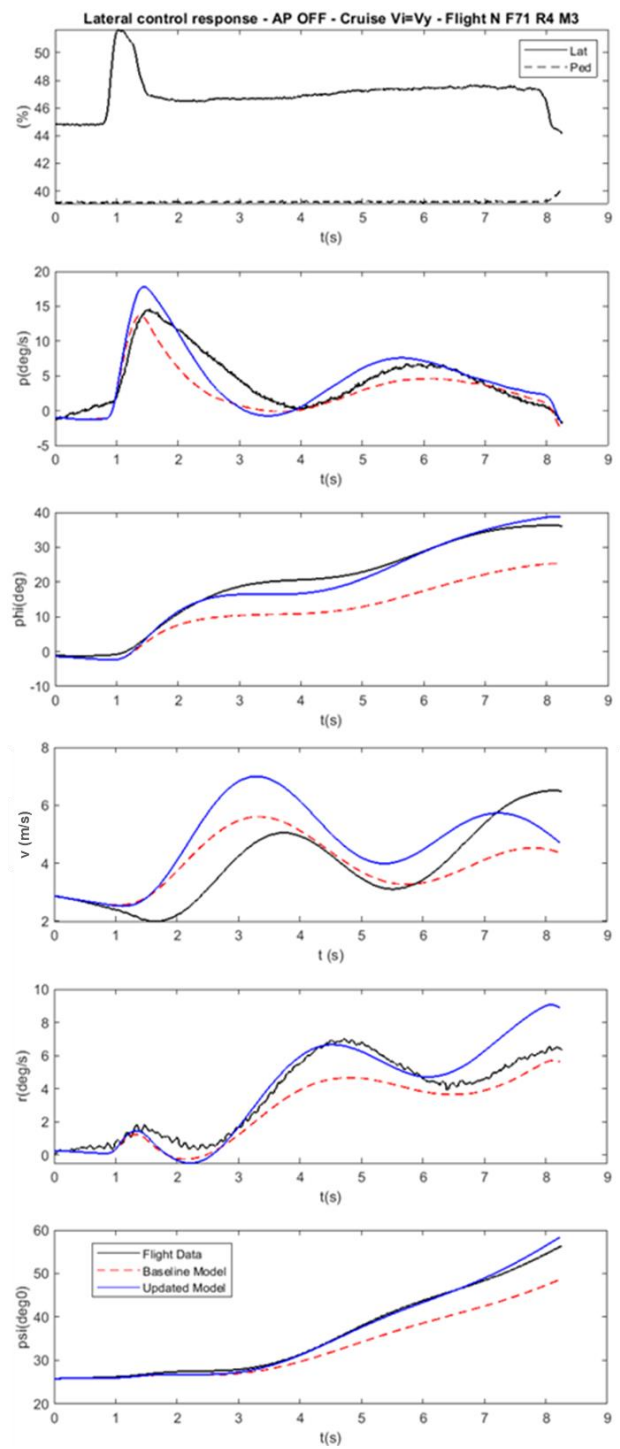
Figure 14. Flight case 4 - comparison with FT, before and after force and moment corrections
