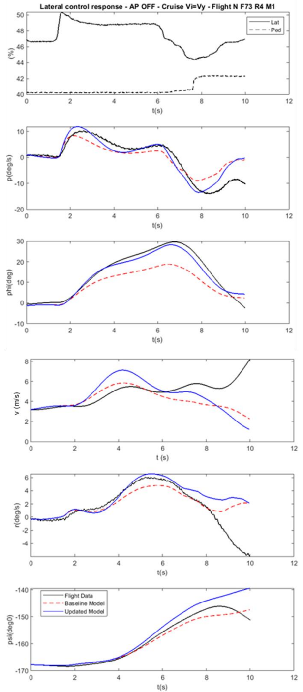
Figure 12. Flight case 2 - comparison with FT, before and after force and moment corrections
