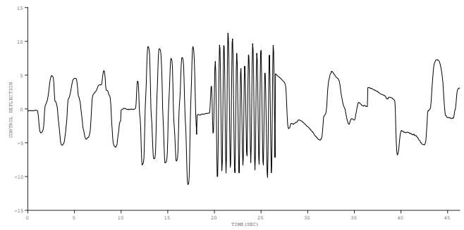
Figure 3. Lateral stick inputs ( \delta_{lat}, \% ) for 5 QTG flight-test records
