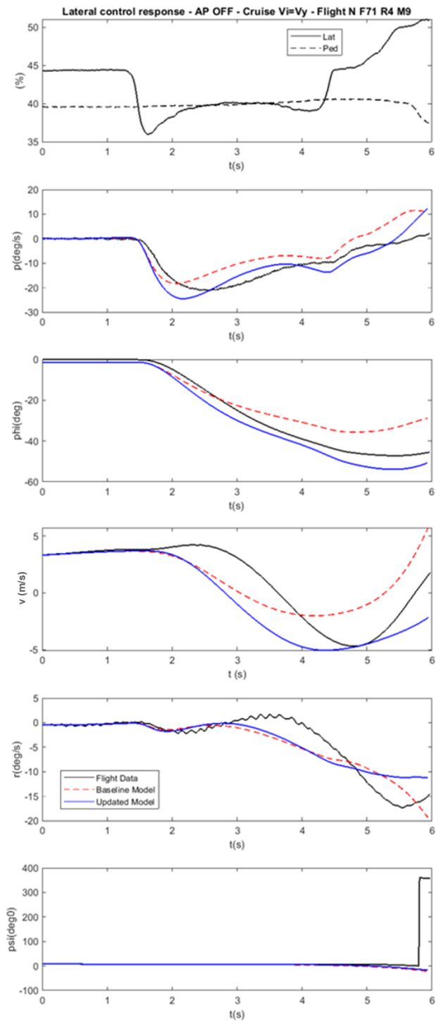
Figure 13. Flight case 3 - comparison with FT, before and after force and moment corrections
