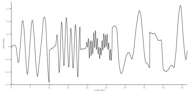
Figure 4. Roll rate response ( p, \text{rad/sec} ) for 5 QTG flight-test records.
