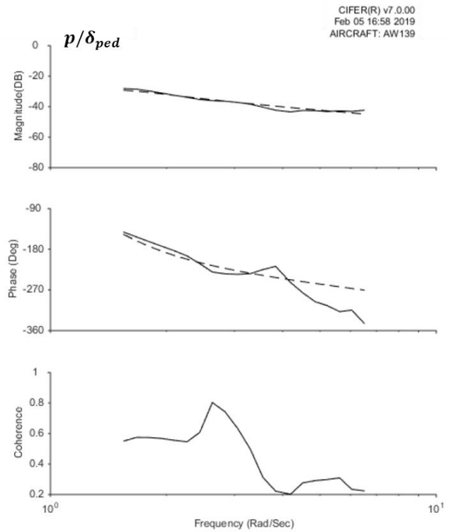
Figure 7. Lateral-directional frequency response – roll rate to pedals
