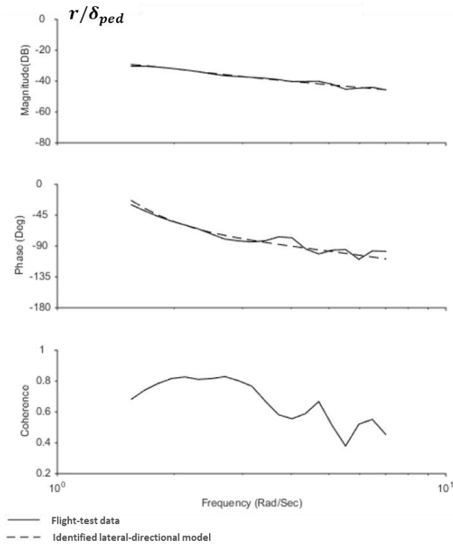
Figure 8. Lateral-directional frequency response – yaw rate to pedals
