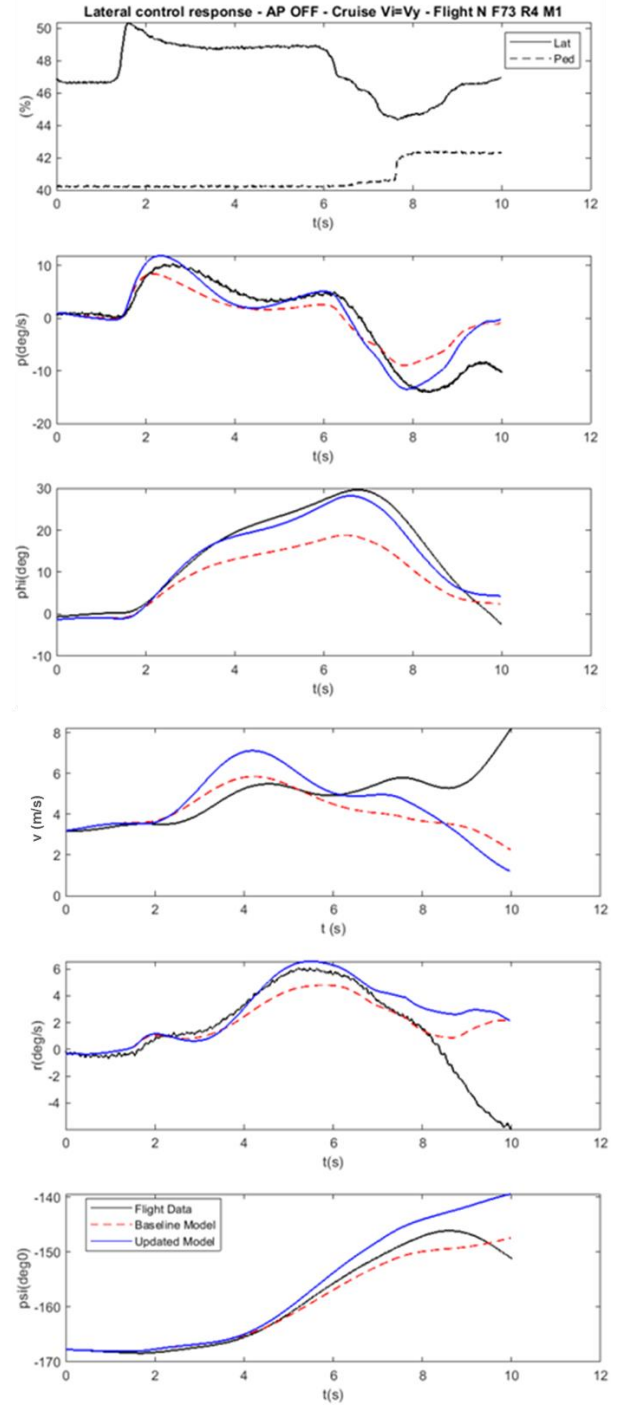
Figure 12. Flight case 2 - comparison with FT, before and after force and moment corrections
