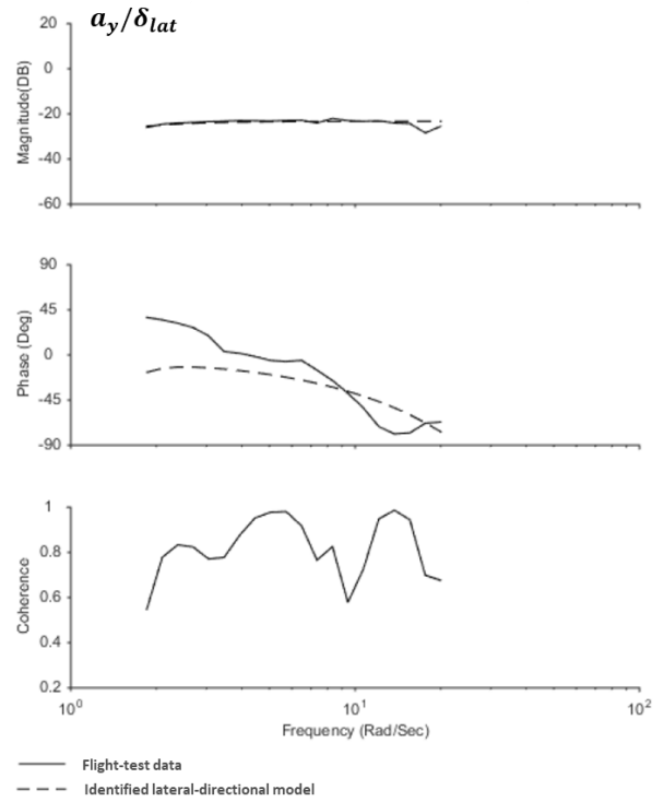
Figure 6. Lateral-directional frequency response – lateral acceleration to lateral stick
