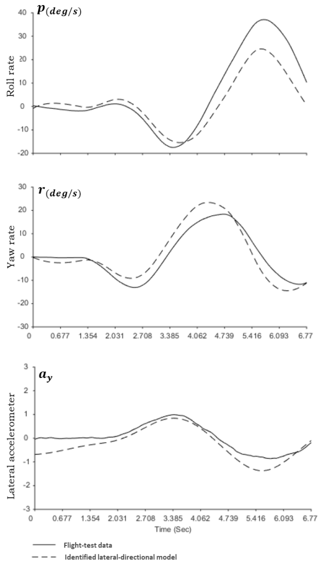
Figure 10. Lateral-directional model time-domain verification agreement for a pedal input
