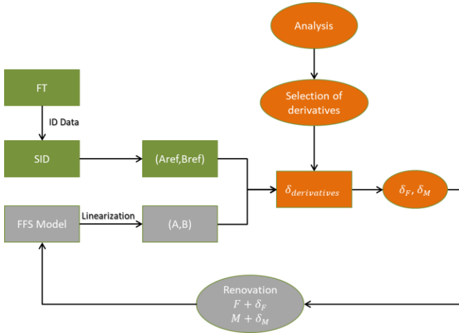
Figure 2. The renovation method by force and moment increments
