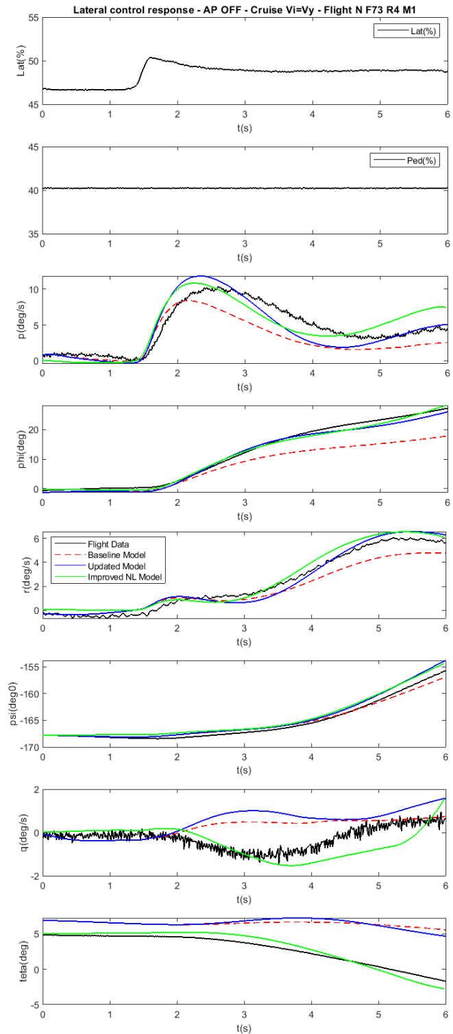
Figure 16. Flight case 2 - comparison with FT, after physics-based model improvement
