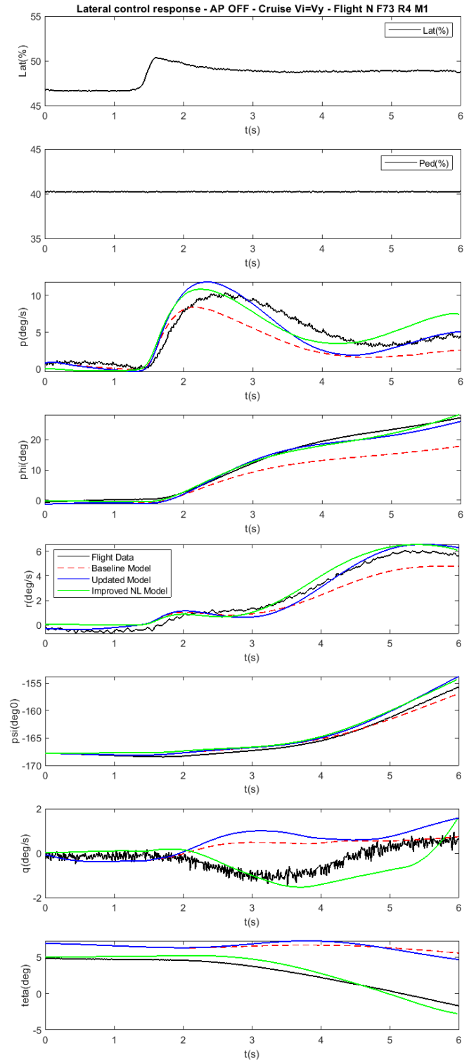
Figure 16. Flight case 2 - comparison with FT, after physics-based model improvement
