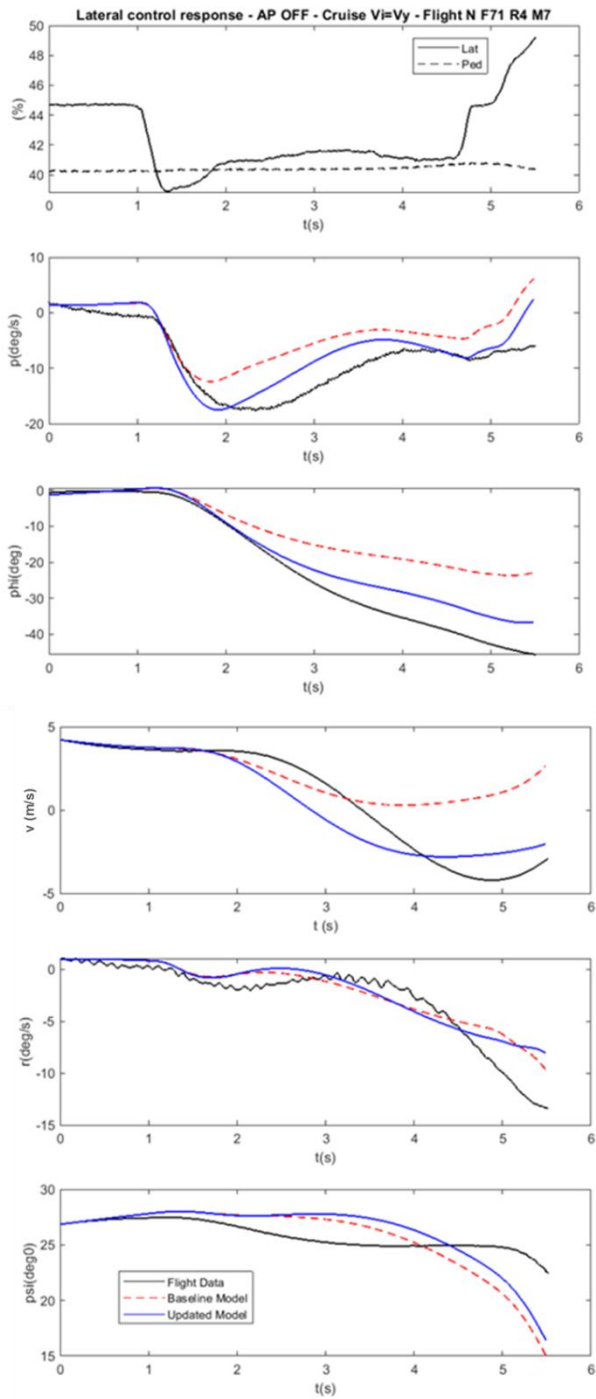
Figure 11. Flight case 1 - comparison with FT, before and after force and moment corrections
