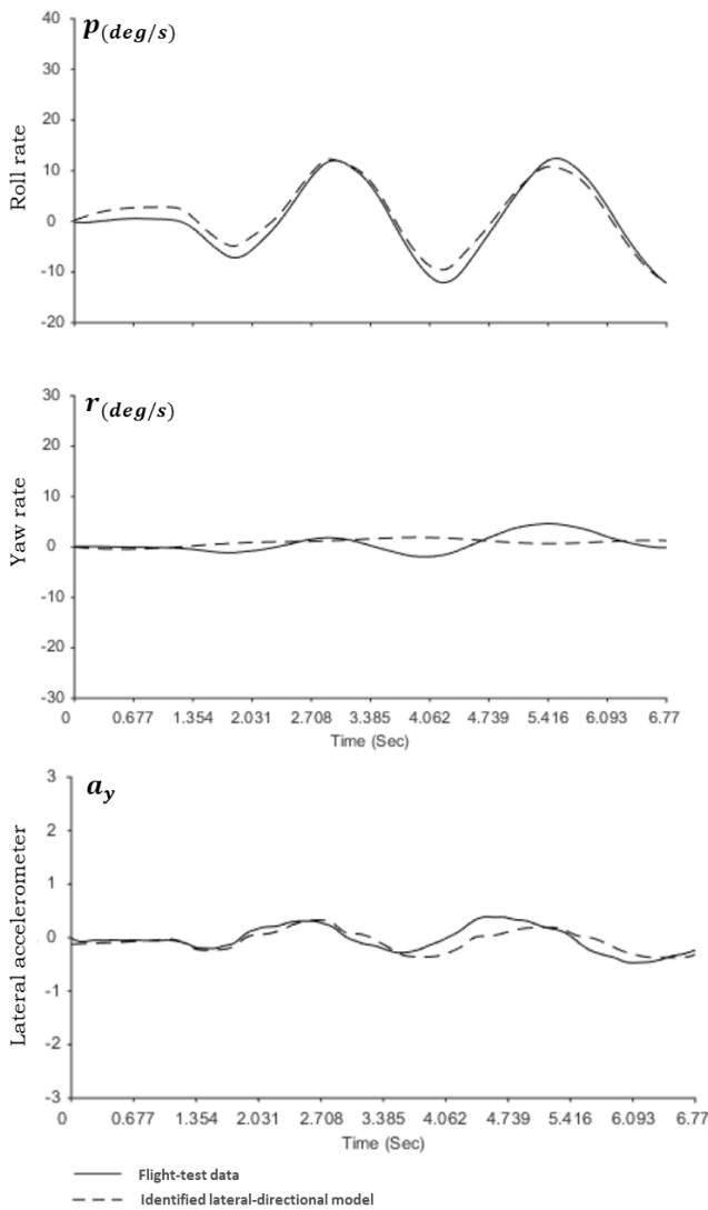
Figure 9. Lateral-directional model time-domain verification agreement for a lateral stick input
