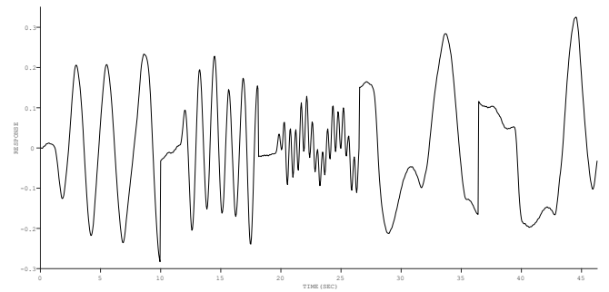
Figure 4. Roll rate response ( p , rad/sec) for 5 QTG flight-test records.
