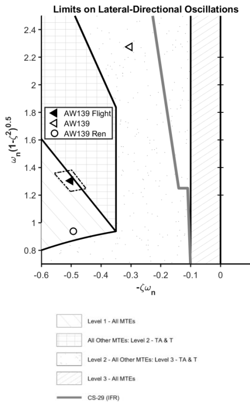
Figure 15. LDO characteristics of AW139 before and after renovation compared with flight
