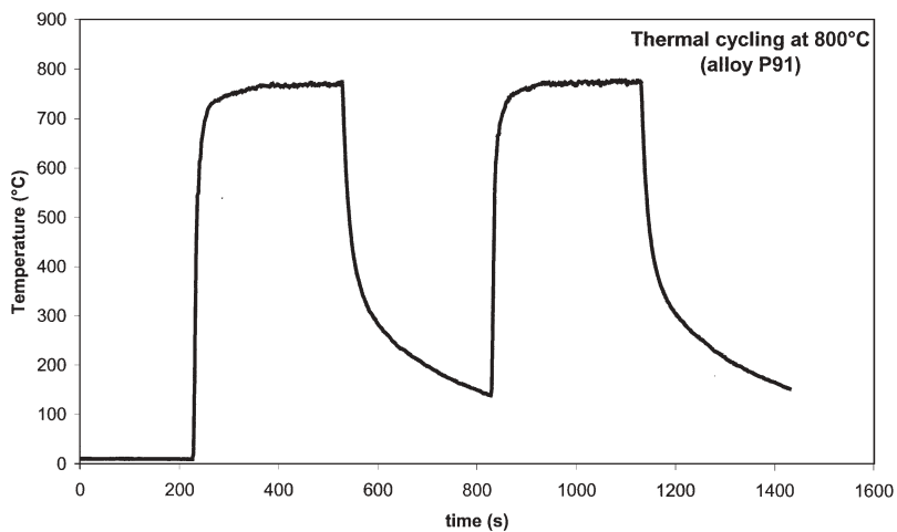
Fig. 7. First two thermal cycles of sample P91 ( 20 \times 10 \times 1 mm). High heating and cooling rates are obtained with a specifically designed thermobalance combining microbalances and a lamp furnace of 6 \times 1000 W allowing the simultaneous cyclic oxidation of 6 samples under controlled atmosphere (see text).
