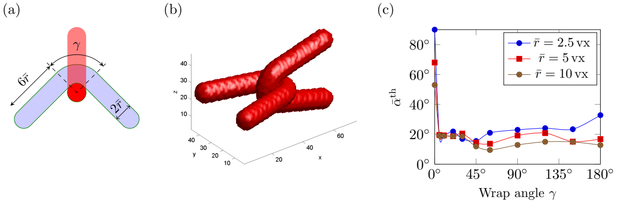
Figure 15: Separation of wavy touching fibres: (a) schematic view of the synthetic geometry, introducing the wrap angle and (b) example of geometry with \gamma = 150^\circ and r = 10 \text{ vx} ; highest values of \bar{\alpha}^{\text{th}} leading to the separation of the fibres wrap around each other, as functions of wrap angle mean fibre radius.
