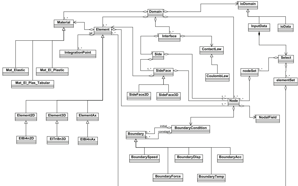
Fig. 2. Simplified UML diagram of the object oriented framework.
