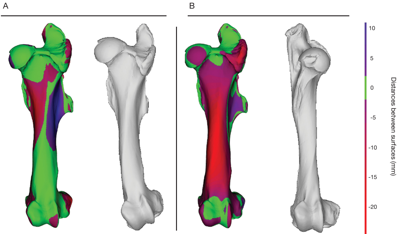
FIG. 3. — Heatmaps of highest distances measured for horse retrodeformed femora from (A) bending and (B) twisting. The distances between the surfaces of the undeformed and a retrodeformed femora were shown directly onto the surface of the original as heatmaps. Bones with the simulated taphonomic deformations were represented in grey.
