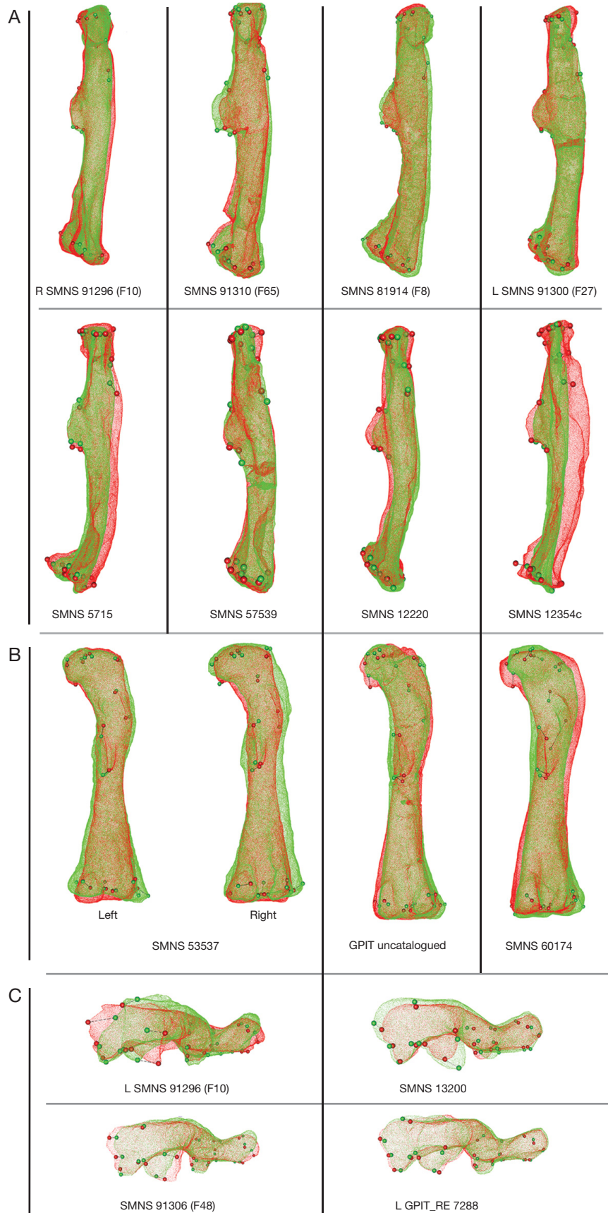
FIG. 6. — Retrodeformations of prosauropod femora in: A , lateral view; B , posterior view; C , 3D distal view. Original bones are shown in green whereas retrodeformed ones are in red. Landmarks of each bone are indicated with the same colours.
