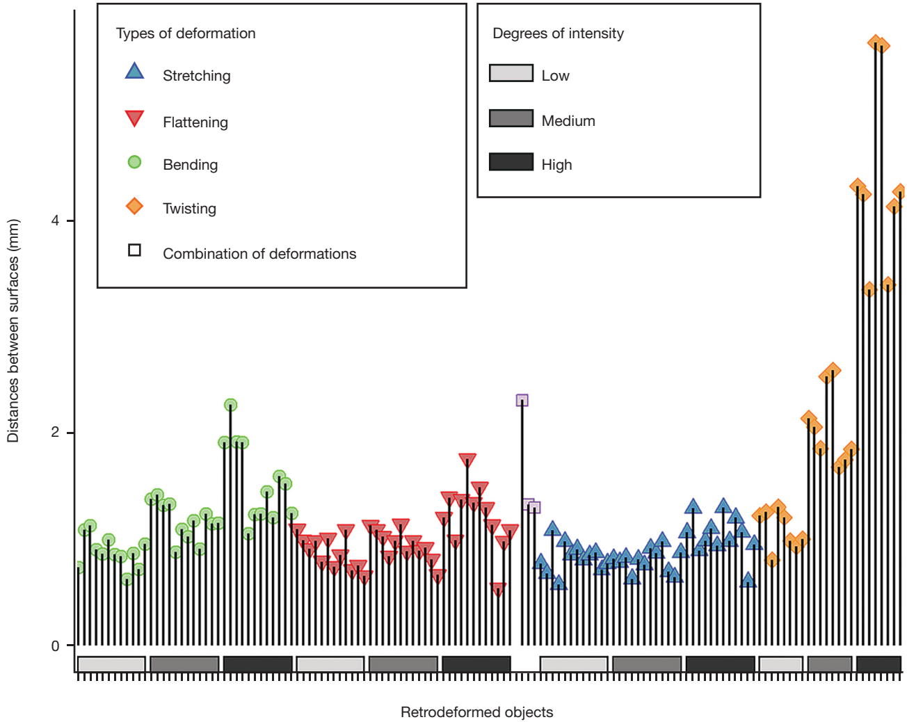
APPENDIX 1. — Distances between the horse original bone and every retrodeformed one. All retrodeformed bones are plotted in abscissa with their associated distances with the original (inter-quartile distance) in ordinate. Types of deformation are represented by the coloured geometrical shapes . Intensities of deformations are figured by rectangles increasingly filled along abscissa.
