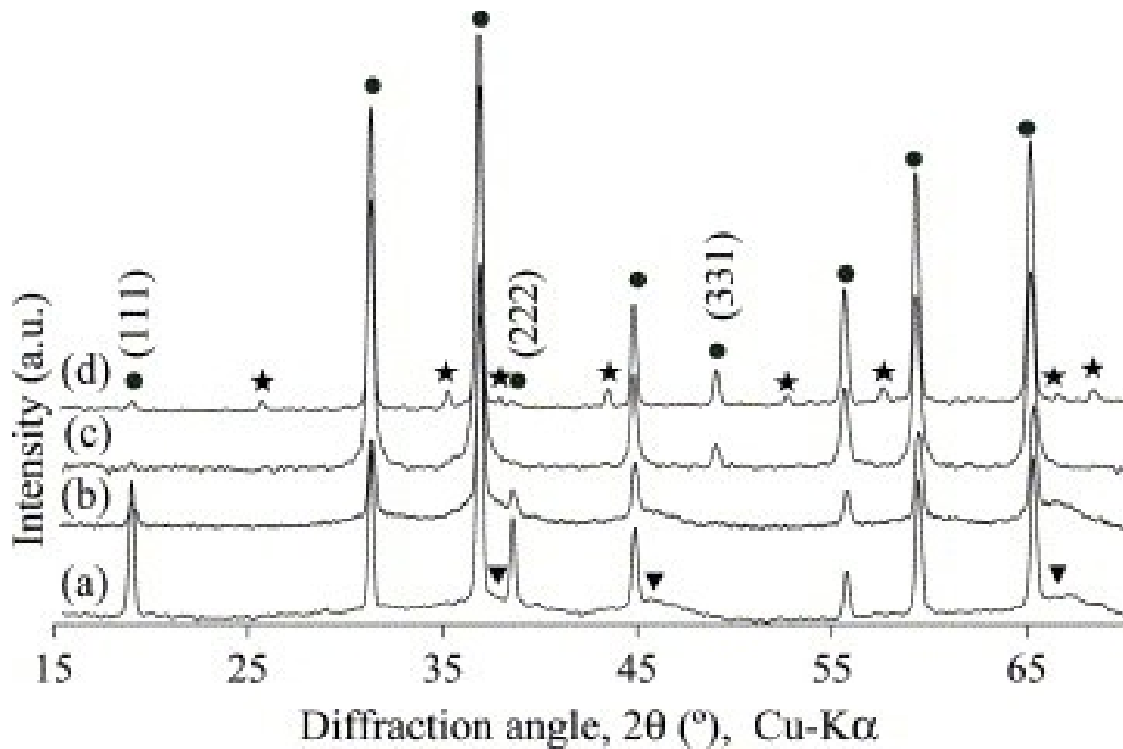
Fig. 1. XRD pattern of samples MS450 (a), MS800 (b), MS1000 (c) and MS1200 (d) —★ \alpha\text{-Al}_2\text{O}_3 , ▼ \gamma\text{-Al}_2\text{O}_3 , ● \text{CoAl}_2\text{O}_4 and \text{Co}_3\text{O}_4 .
