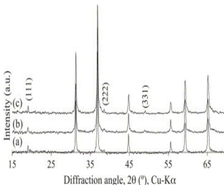
Fig. 8. XRD pattern of samples CL800 (a), CL1000 (b) and CL1200 (c).
