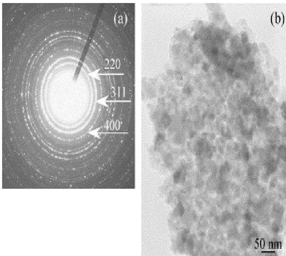
Fig. 5. Electron diffraction pattern (a) and electron micrograph (b) of sample MS1000.
