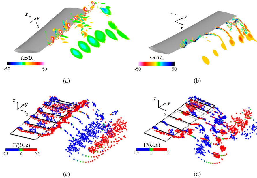
FIG. 20: Spanwise vorticity fields for t/T = 0.25 for the flexible (top) and highly flexible (bottom) wings; Re = 30,000 , k_G = 1.82 : dimensionless vorticity \Omega c/U_\infty contours plotted from computations downstream of the trailing edge 12 : (a) flexible, Reproduced with permission from J. Fluids Struct. 40 (2013). Copyright 2013 Elsevier, (b) highly flexible, Reproduced with permission from J. Fluids Struct. 40 (2013). Copyright 2013 Elsevier, dimensionless circulation \Gamma/(U_\infty c) vortical centers from LDVM simulation: (c) flexible, (d) highly flexible. The six spanwise visualization sections ( y/c = 0.5, 1, 1.5, 2, 2.5, 2.85 ) are identical for the computations downstream of the trailing edge 12 and LDVM simulations.
