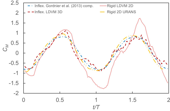
FIG. 10: Comparison for the inflexible wing, of the time histories of the quarter-chord pitching moment coefficient from computational results of Gordnier et al. 12 with present study results of the 2D URANS, 2D LDVM and 3D LDVM.
