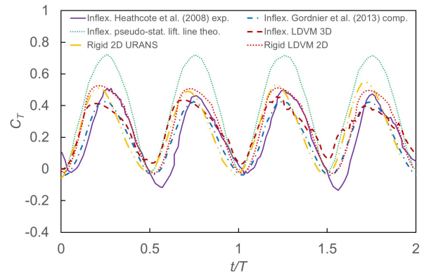
FIG. 8: Comparison for the inflexible wing, of the time histories of the thrust coefficient from experimental results of Heathcote et al. 11 and computational results of Gordnier et al. 12 with present study results of the pseudo-stationary lifting line theory, 2D URANS, 2D LDVM and 3D LDVM.
