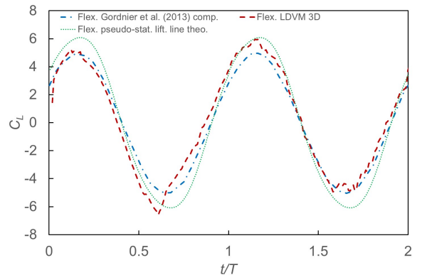
FIG. 12: Comparison for the flexible wing, of the time histories of the lift coefficient from computational results of Gordnier et al. 12 with present study results of the pseudo-stationary lifting line theory and 3D LDVM.
