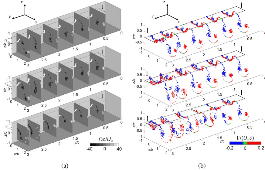
FIG. 18: Spanwise vorticity fields for t/T = 0.25 for the inflexible (top), flexible (middle), and highly flexible (bottom) wings; Re = 30,000 , k_G = 1.82 : (a) dimensionless vorticity \Omega c/U_\infty contours plotted from PIV measurements downstream of the trailing edge 11 Reproduced with permission from J. Fluids Struct. 24 (2008). Copyright 2008 Elsevier, (b) dimensionless circulation \Gamma/(U_\infty c) vortical centers from LDVM simulation. The six spanwise visualization sections ( y/c = 0.5, 1, 1.5, 2, 2.5, 2.85 ) are identical for the PIV measurements and LDVM simulations.
