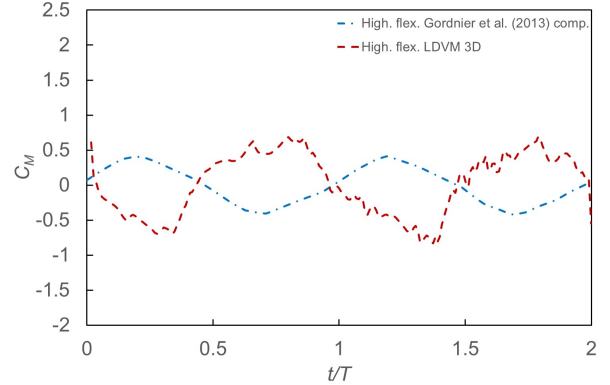
FIG. 16: Comparison for the highly flexible wing, of the time histories of the quarter-chord pitching moment coefficient from computational results of Gordnier et al. 12 with present study results of 3D LDVM.
