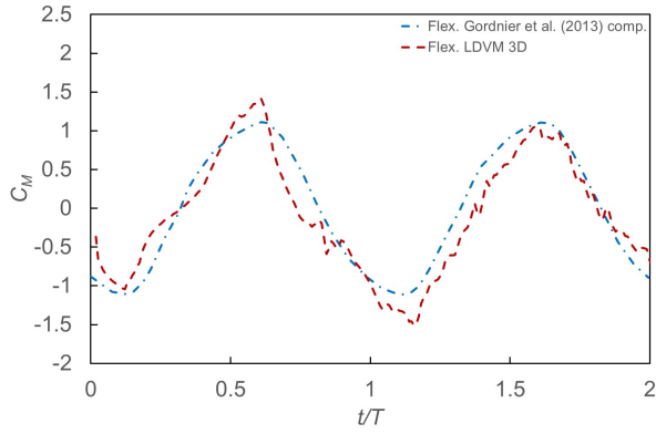
FIG. 13: Comparison for the flexible wing, of the time histories of the quarter-chord pitching moment coefficient from computational results of Gordnier et al. 12 with present study results of the 3D LDVM.
