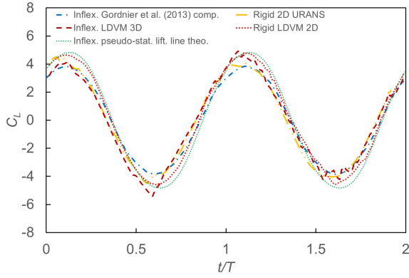
FIG. 9: Comparison for the inflexible wing, of the time histories of the lift coefficient from computational results of Gordnier et al. 12 with present study results of the pseudo-stationary lifting line theory, 2D URANS, 2D LDVM and 3D LDVM.
