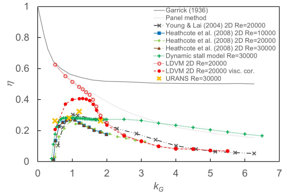
FIG. 5: Comparison of propulsive efficiency versus Garrick frequency k_G for a NACA0012 airfoil in pure heave, for present study dynamic stall model, LDVM and URANS with published data of linear theory (Garrick 6 ), panel method, Navier-Stokes solver (Young & Lai 9 ) and experiment (Heathcote et al. 11 ).
