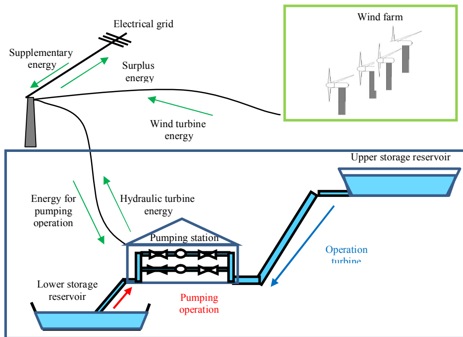
Figure 3. Hybrid pumped hydro/wind energy
