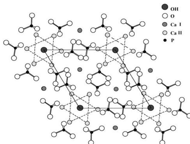
Fig. 1. Projection on the (001) plane of the hydroxyapatite structure. The two \text{Ca}^{2+} triangles lining the “tunnels” of the structure are located at z 1/4 and z 3/4. \text{OH}^- ions are slightly under or above the triangles.
