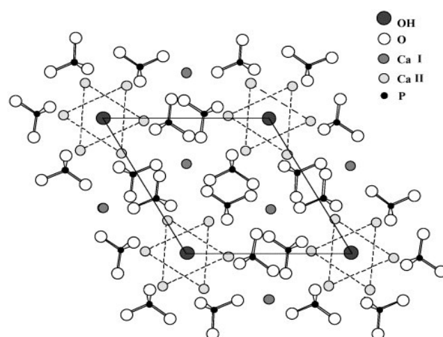
Fig. 1. Projection on the (001) plane of the hydroxyapatite structure. The two \text{Ca}^{2+} triangles lining the “tunnels” of the structure are located at z\ 1/4 and z\ 3/4 . \text{OH}^- ions are slightly under or above the triangles.
