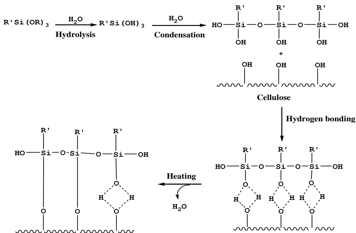
Figure 1: Mechanism of chemical treatment of cellulose fibers with a trialkoxysilane.
