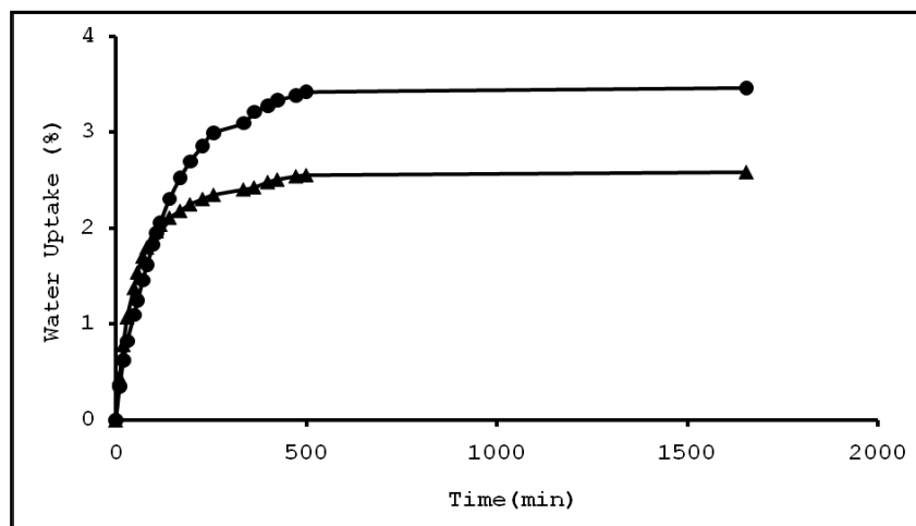
Figure 3: Moisture uptake percentage versus time of CF (●) and mCF (▲) .
