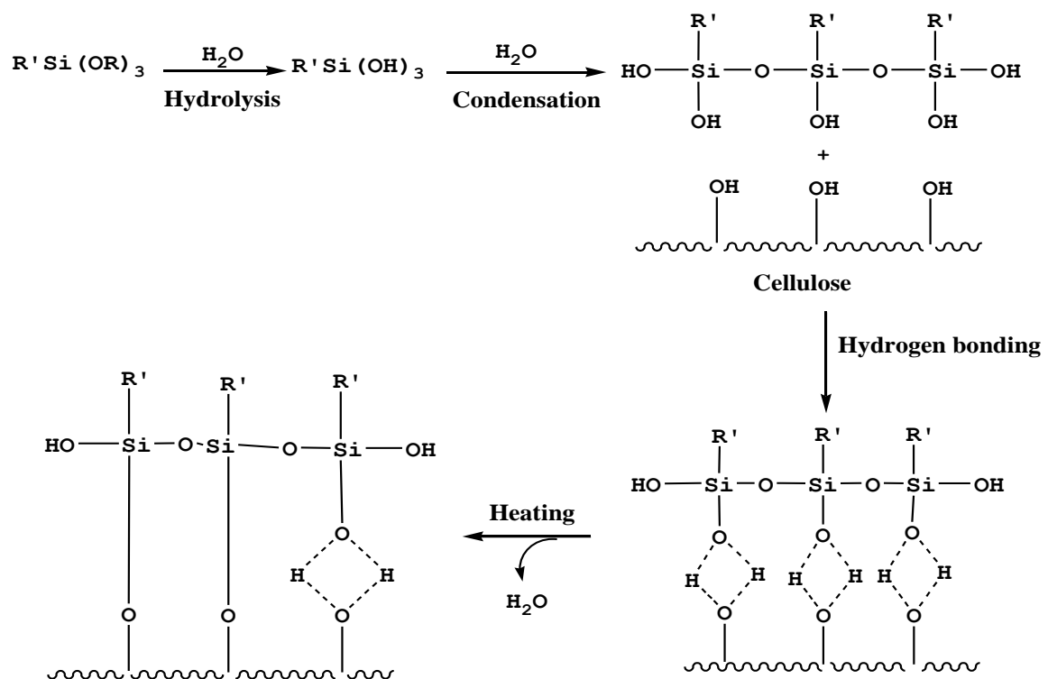
Figure 1: Mechanism of chemical treatment of cellulose fibers with a trialkoxysilane.
