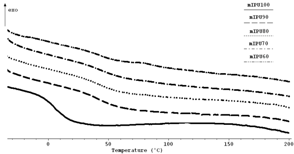
Figure 8 : DSC thermograms IPUi and mIPUi versus fiber percentage.
