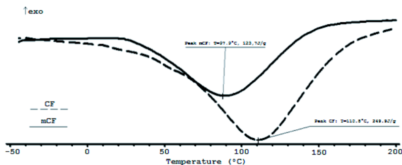
Figure 4: First scan DSC curves of CF and mCF.
