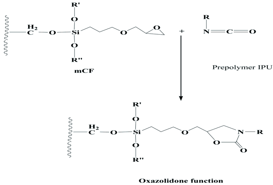
Figure 7 : Oxazolidone formation by reaction between glycidyl and isocyanate groups
