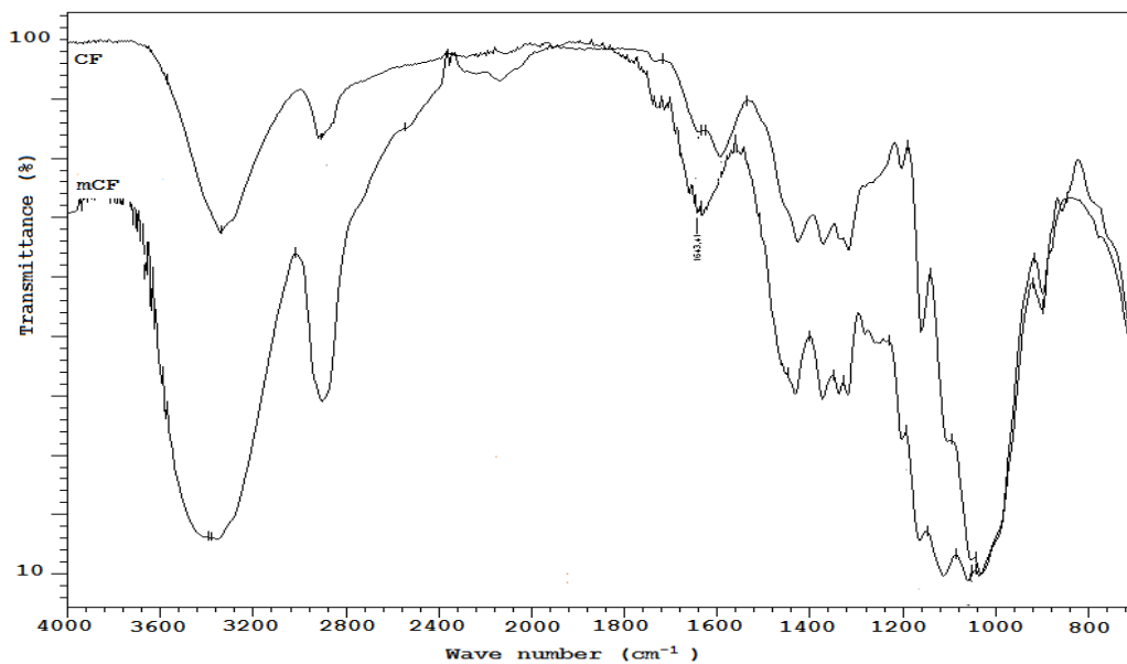
Figure 2: ATR-FTIR of CF and mCF.
