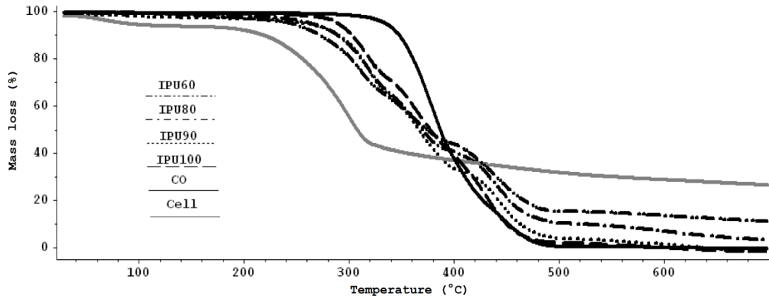
Figure 9: TGA thermograms of CO, mCF and mIPUi.
