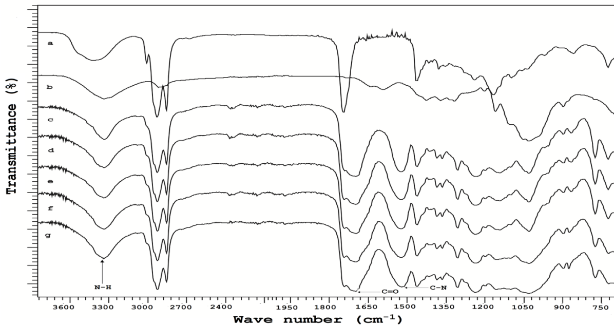
Figure 6: ATR-FTIR spectra of (a) CO, (b) mIPU100, (c) mIPU80, (d) mIPU60 and (e) mCF.
