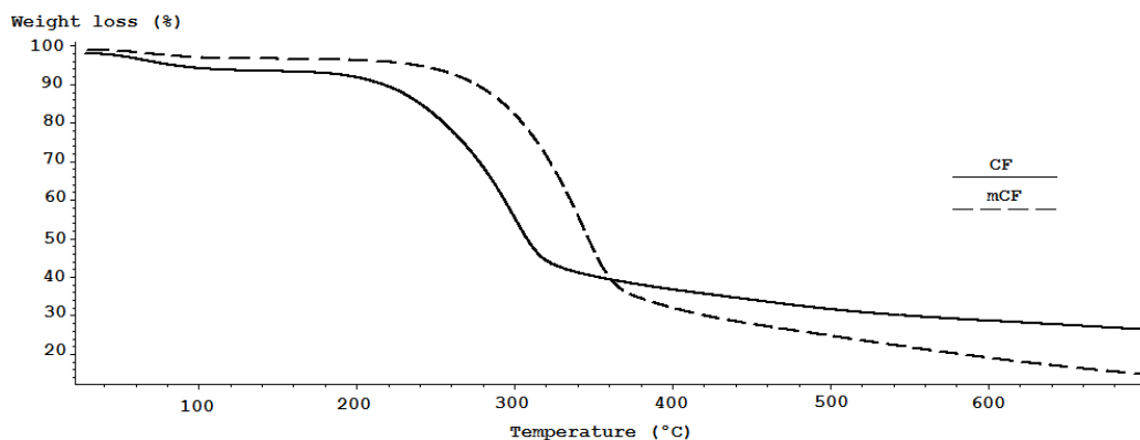
Figure 5: TGA and DTG thermograms of CF and mCF.
