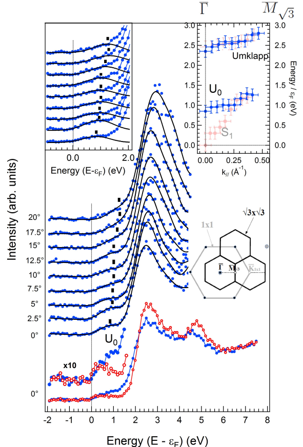
FIG. 3: (color online). Kripes spectra of the Si layer deposited on \sqrt{3} -Ag surface, for increasing incidence angle \theta along the \bar{\Gamma} - \bar{M}\sqrt{3} direction. At the bottom the NI spectrum before Si deposition (red open circles) is also reported for comparison with the normal incidence IPE spectrum after Si deposition (blue filled circles). The upper panels are like in Fig. 2 and the dispersion of the S_1 state (pink shaded circles) is reported in the top-right panel for comparison. The unreconstructed Si(111)- 1 \times 1 and \sqrt{3} \times \sqrt{3} surface Brillouin zones are also depicted to highlight the coincidence between \bar{K}_{1 \times 1} and \bar{\Gamma}\sqrt{3 \times \sqrt{3}} .
