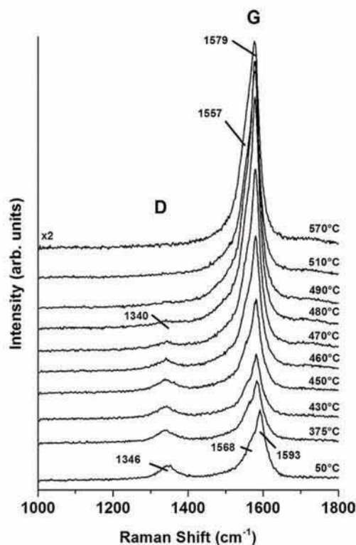
Fig. 1. In situ Raman spectroscopy study of the changes in the D and G band of DWCNT during oxidation (514.5 nm laser excitation wavelength).
