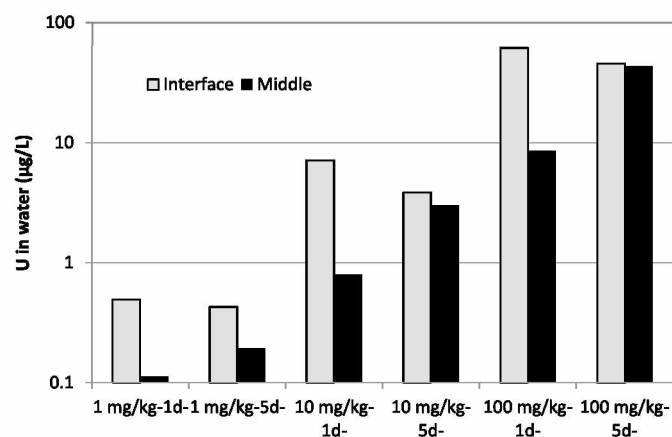
Fig. 1. Uranium concentration (µg L -1 , n = 1) in water at various depths (interface and mid-water column) for 3 spiked-sediment after 1 and 5 days.
