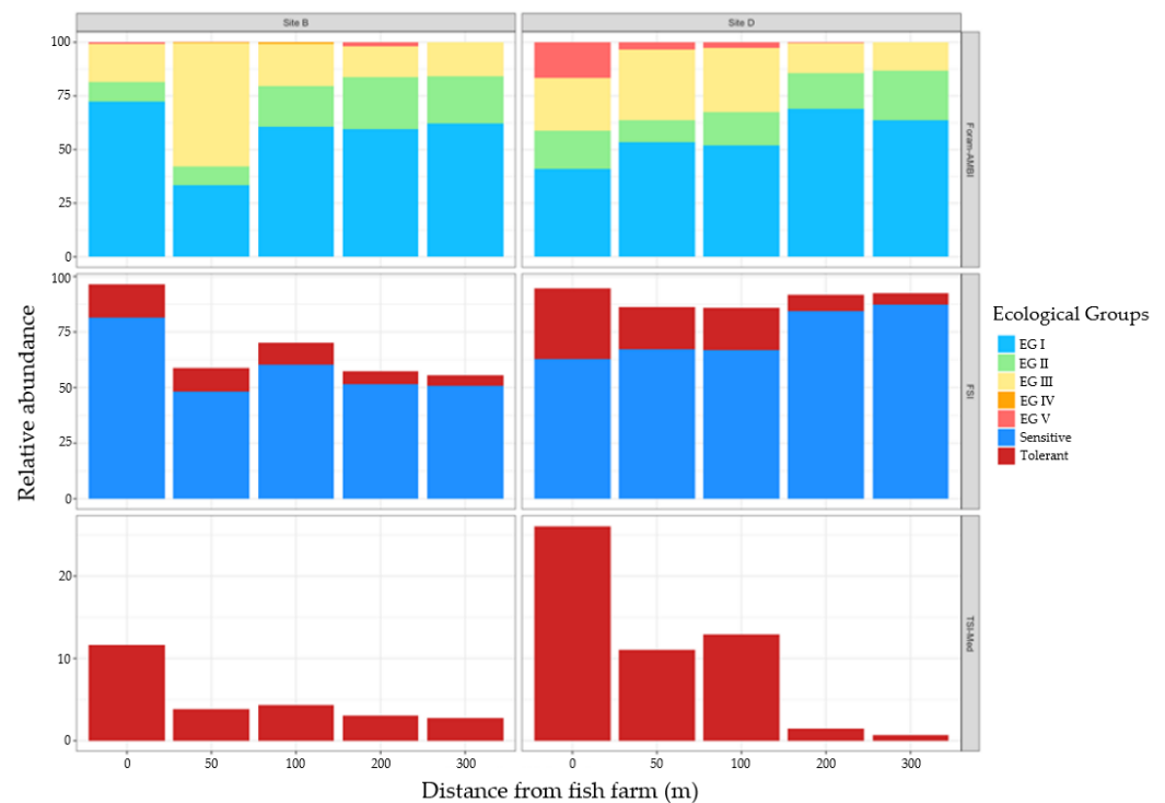
Figure 8. Relative proportion of the different groups of indicative species as defined and classified by the authors: EGI, EGII, EGIII, EGIV and EGV, for Forams-AMBI [47]; group of tolerant and sensitive species for FSI [49]; group of tolerant species for TSI-Med [31,48].
