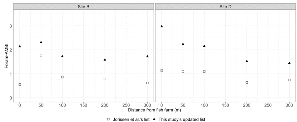
Figure 10. Comparison of Foram-AMBI values according to [47] and the study-updated list.
